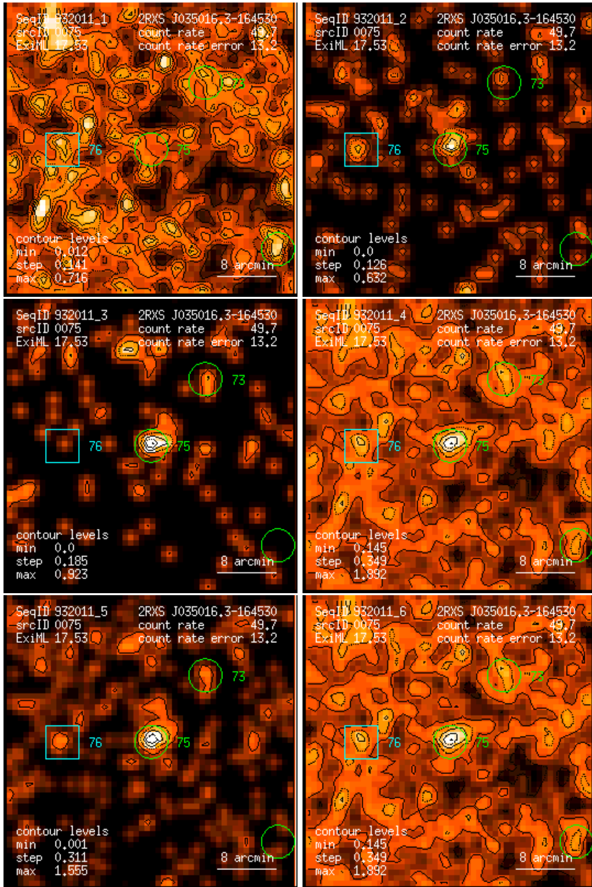
Figure 75: RASS 932011: detection 0075: band rate images, Gaussian filter: (1) PSPC channels 11 – 41, (2) 52 – 90, (3) 91 – 201, (4) 11 – 235, (5) 52 – 201, (6) 11 – 201. Broad band rates in counts/ks. Band rate contour levels in counts/ks/arcmin 2 .
