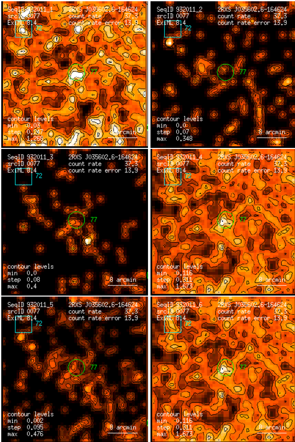
Figure 77: RASS 932011: detection 0077: band rate images, Gaussian filter: (1) PSPC channels 11 – 41, (2) 52 – 90, (3) 91 – 201, (4) 11 – 235, (5) 52 – 201, (6) 11 – 201. Broad band rates in counts/ks. Band rate contour levels in counts/ks/arcmin 2 .
