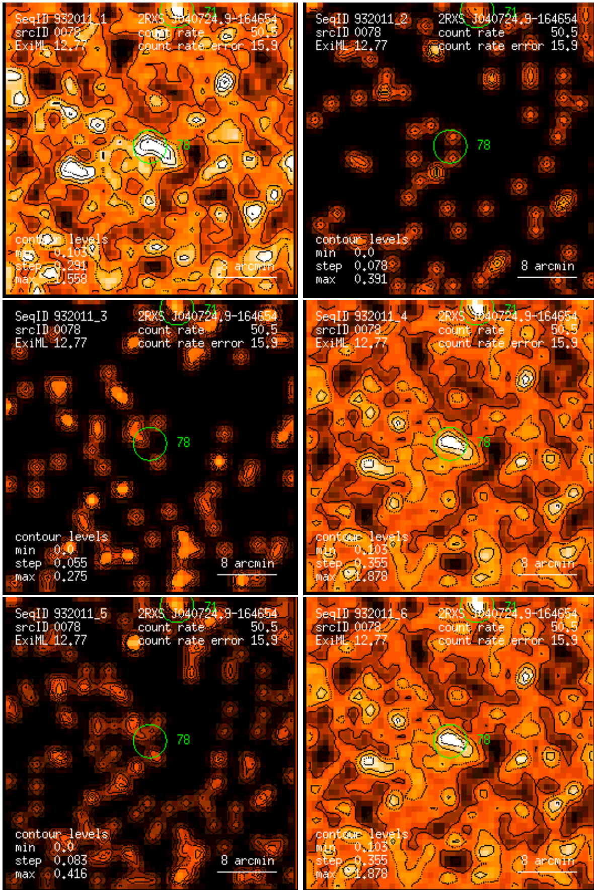
Figure 78: RASS 932011: detection 0078: band rate images, Gaussian filter: (1) PSPC channels 11 – 41, (2) 52 – 90, (3) 91 – 201, (4) 11 – 235, (5) 52 – 201, (6) 11 – 201. Broad band rates in counts/ks. Band rate contour levels in counts/ks/arcmin 2 .
