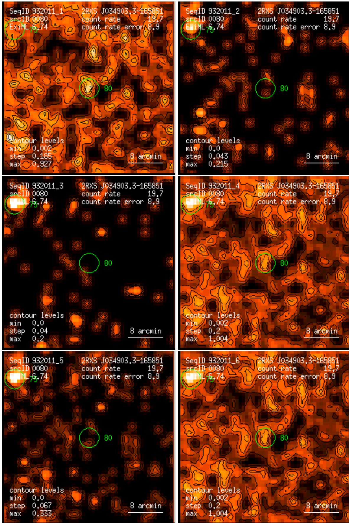
Figure 80: RASS 932011: detection 0080: band rate images, Gaussian filter: (1) PSPC channels 11 – 41, (2) 52 – 90, (3) 91 – 201, (4) 11 – 235, (5) 52 – 201, (6) 11 – 201. Broad band rates in counts/ks. Band rate contour levels in counts/ks/arcmin 2 .
