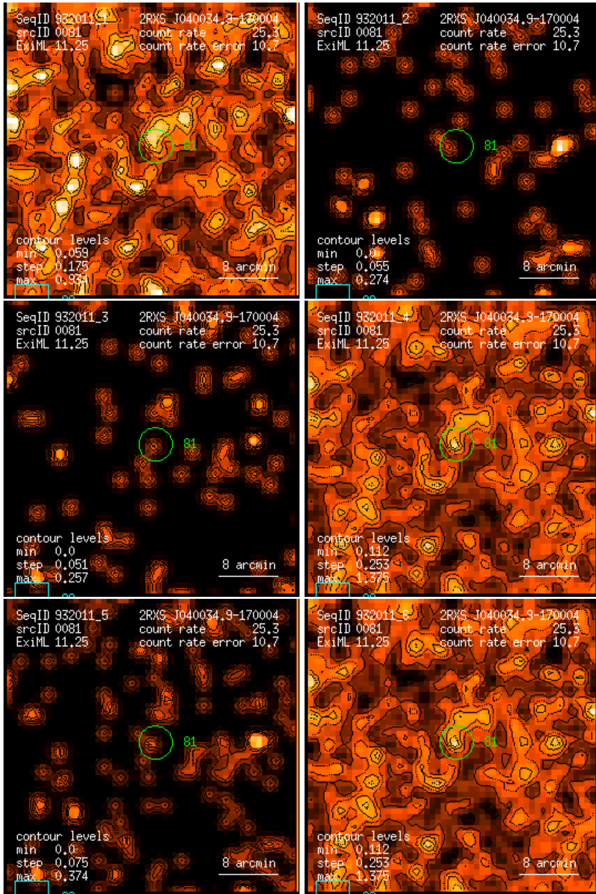
Figure 81: RASS 932011: detection 0081: band rate images, Gaussian filter: (1) PSPC channels 11 – 41, (2) 52 – 90, (3) 91 – 201, (4) 11 – 235, (5) 52 – 201, (6) 11 – 201. Broad band rates in counts/ks. Band rate contour levels in counts/ks/arcmin 2 .
