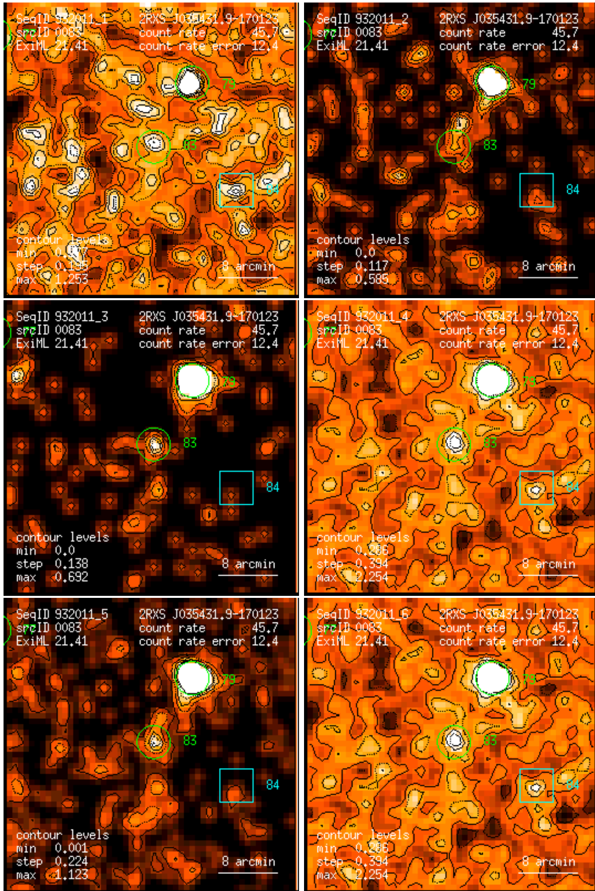
Figure 83: RASS 932011: detection 0083: band rate images, Gaussian filter: (1) PSPC channels 11 – 41, (2) 52 – 90, (3) 91 – 201, (4) 11 – 235, (5) 52 – 201, (6) 11 – 201. Broad band rates in counts/ks. Band rate contour levels in counts/ks/arcmin 2 .
