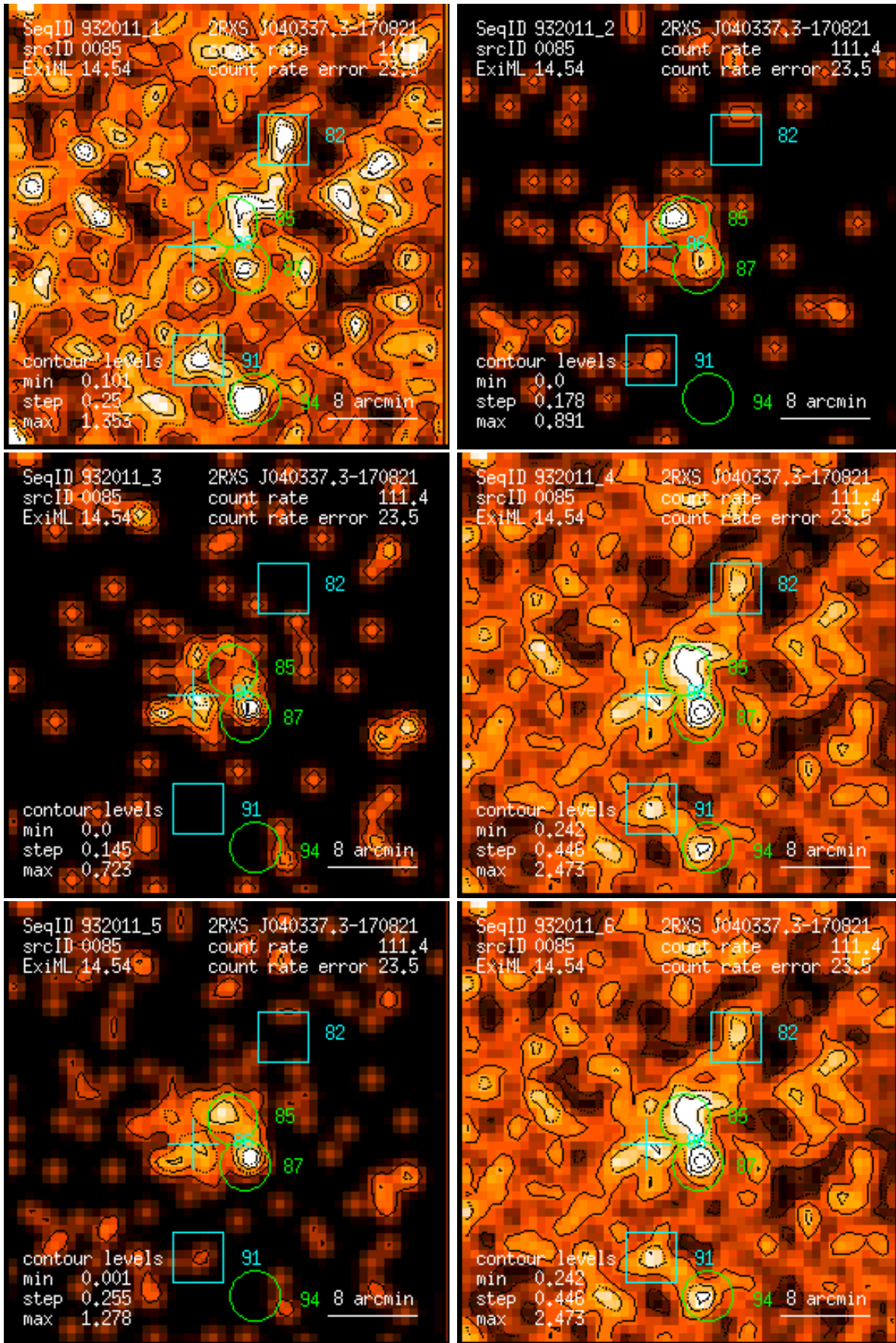
Figure 85: RASS 932011: detection 0085: band rate images, Gaussian filter: (1) PSPC channels 11 – 41, (2) 52 – 90, (3) 91 – 201, (4) 11 – 235, (5) 52 – 201, (6) 11 – 201. Broad band rates in counts/ks. Band rate contour levels in counts/ks/arcmin 2 .
