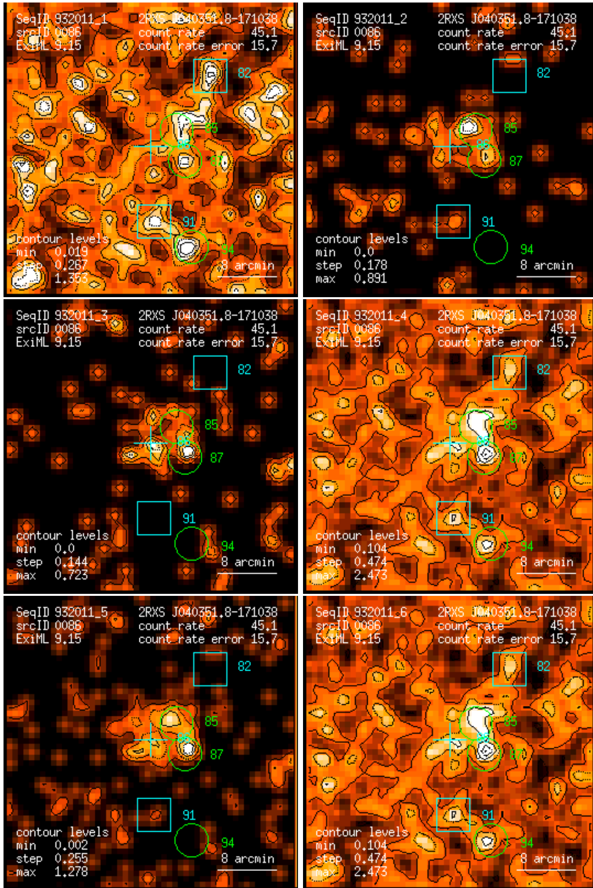
Figure 86: RASS 932011: detection 0086: band rate images, Gaussian filter: (1) PSPC channels 11 – 41, (2) 52 – 90, (3) 91 – 201, (4) 11 – 235, (5) 52 – 201, (6) 11 – 201. Broad band rates in counts/ks. Band rate contour levels in counts/ks/arcmin 2 .
