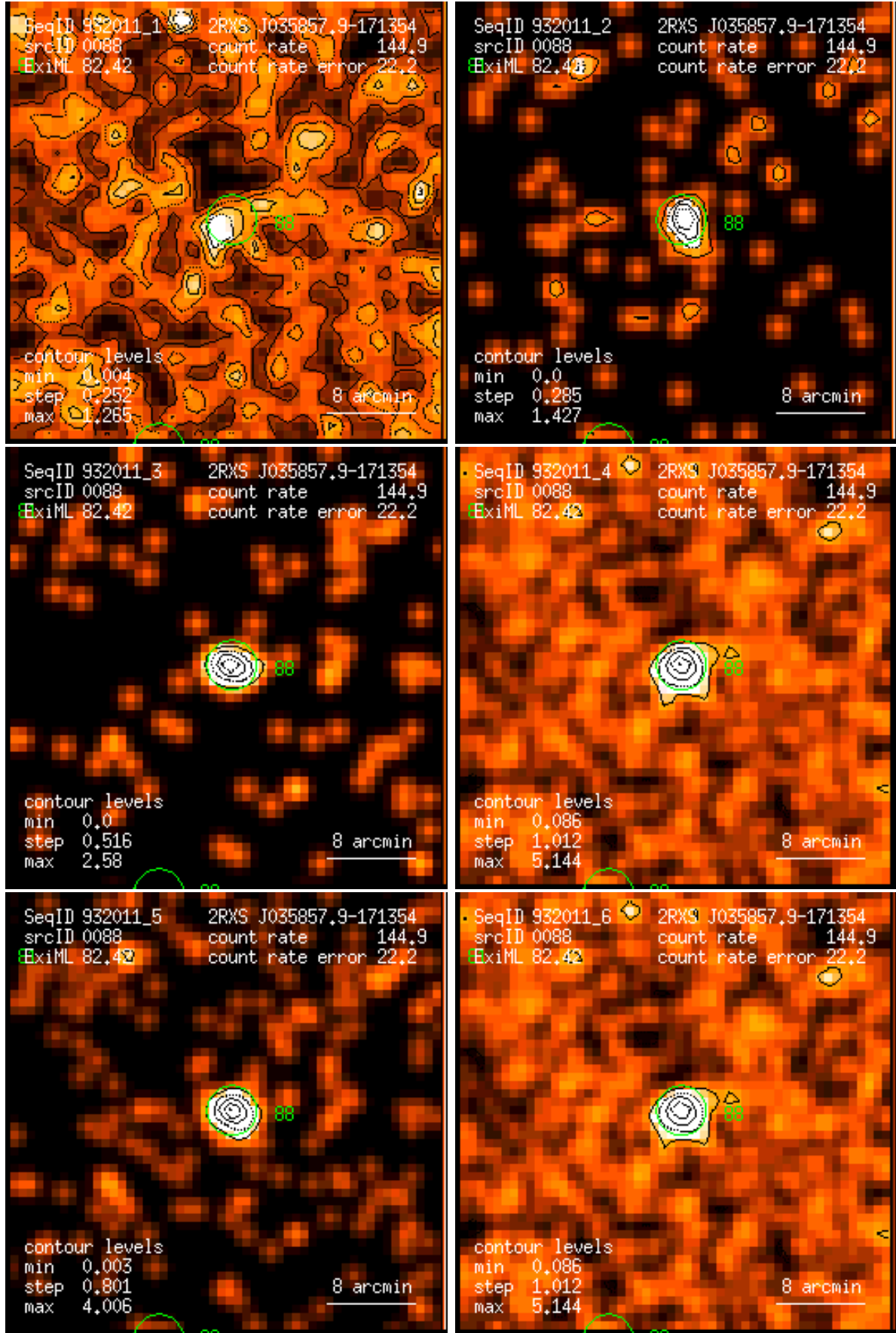
Figure 88: RASS 932011: detection 0088: band rate images, Gaussian filter: (1) PSPC channels 11 – 41, (2) 52 – 90, (3) 91 – 201, (4) 11 – 235, (5) 52 – 201, (6) 11 – 201. Broad band rates in counts/ks. Band rate contour levels in counts/ks/arcmin 2 .
