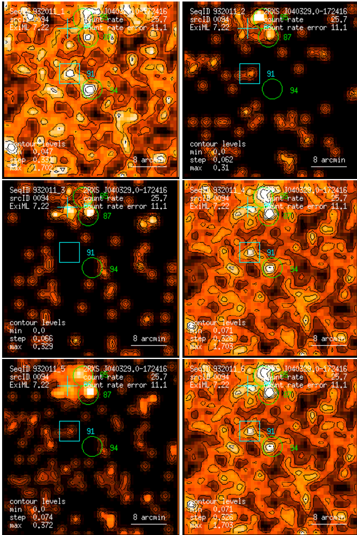
Figure 94: RASS 932011: detection 0094: band rate images, Gaussian filter: (1) PSPC channels 11 – 41, (2) 52 – 90, (3) 91 – 201, (4) 11 – 235, (5) 52 – 201, (6) 11 – 201. Broad band rates in counts/ks. Band rate contour levels in counts/ks/arcmin 2 .
