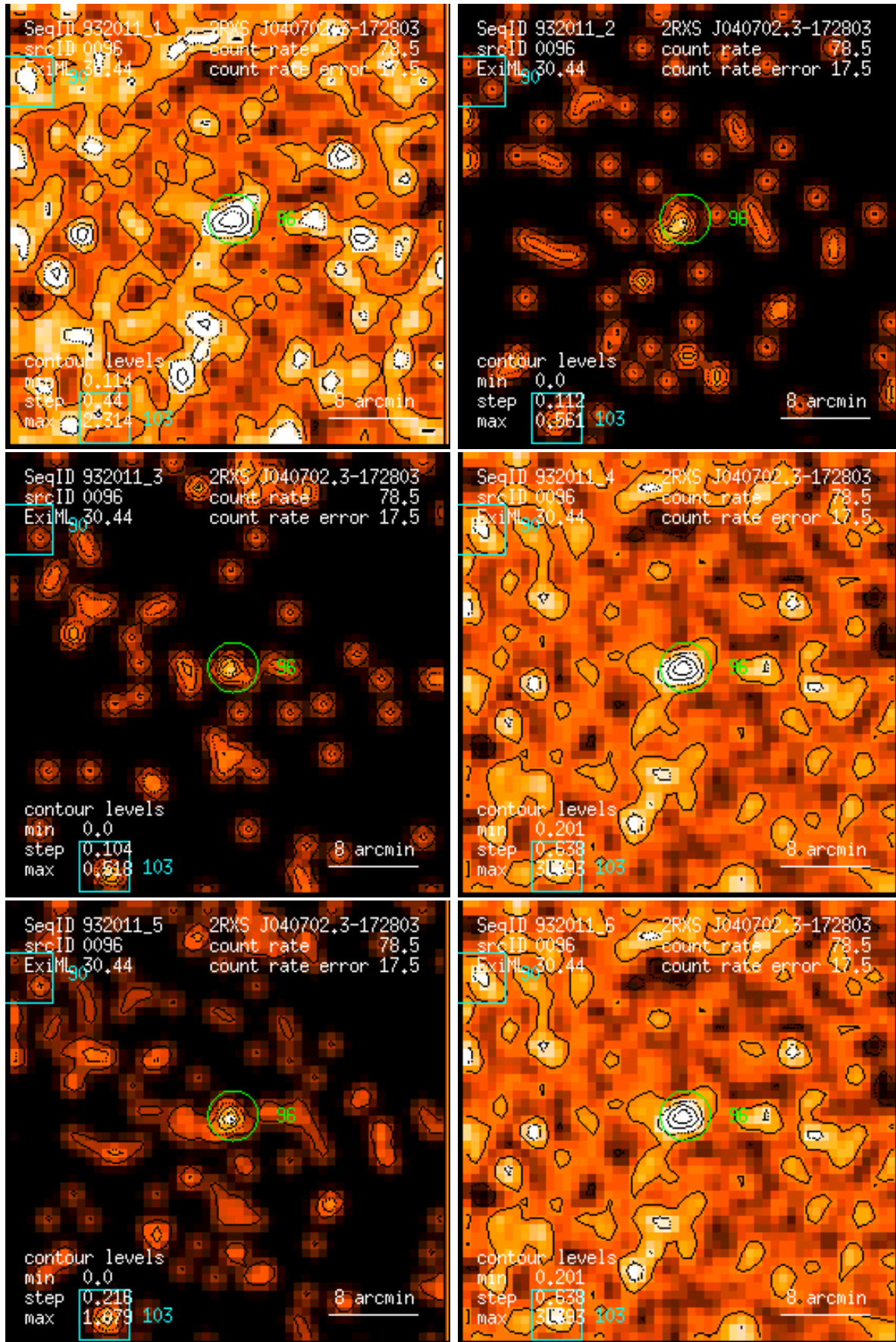
Figure 96: RASS 932011: detection 0096: band rate images, Gaussian filter: (1) PSPC channels 11 – 41, (2) 52 – 90, (3) 91 – 201, (4) 11 – 235, (5) 52 – 201, (6) 11 – 201. Broad band rates in counts/ks. Band rate contour levels in counts/ks/arcmin 2 .
