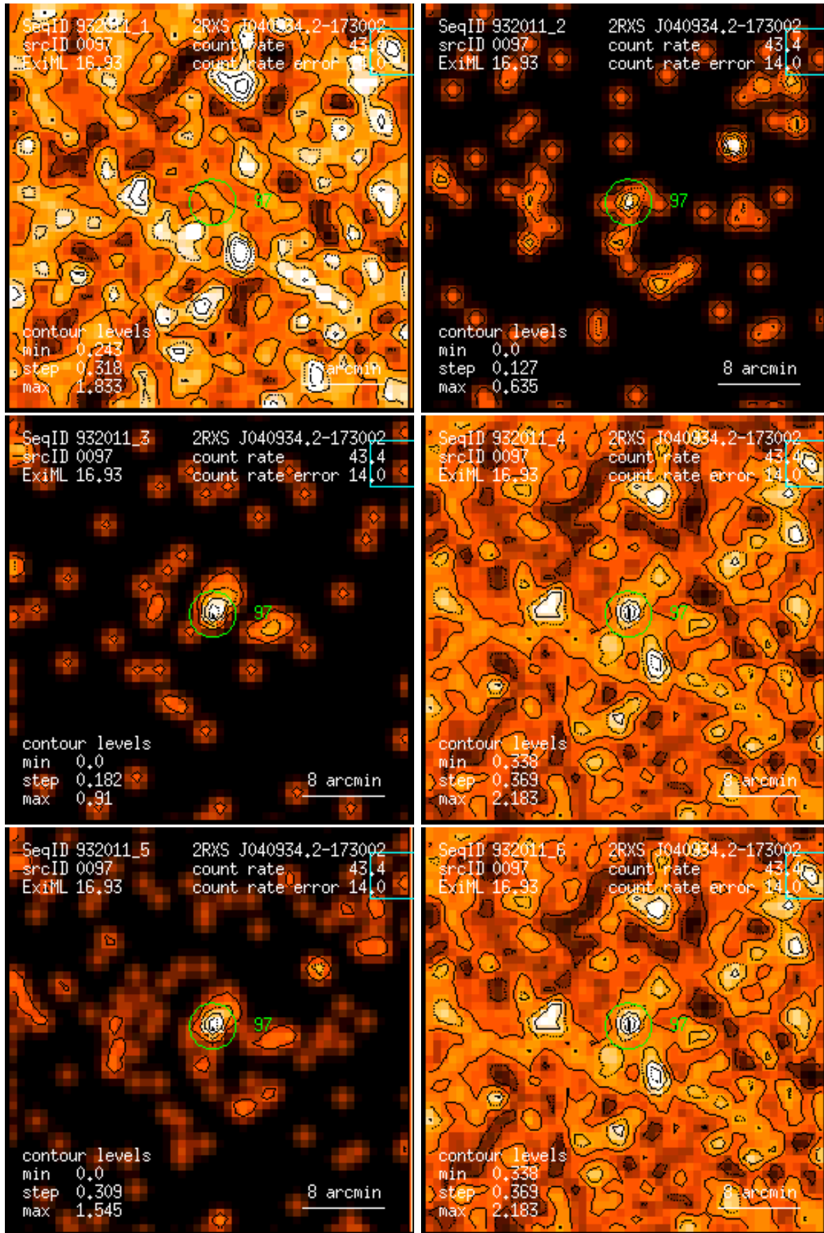
Figure 97: RASS 932011: detection 0097: band rate images, Gaussian filter: (1) PSPC channels 11 – 41, (2) 52 – 90, (3) 91 – 201, (4) 11 – 235, (5) 52 – 201, (6) 11 – 201. Broad band rates in counts/ks. Band rate contour levels in counts/ks/arcmin 2 .
