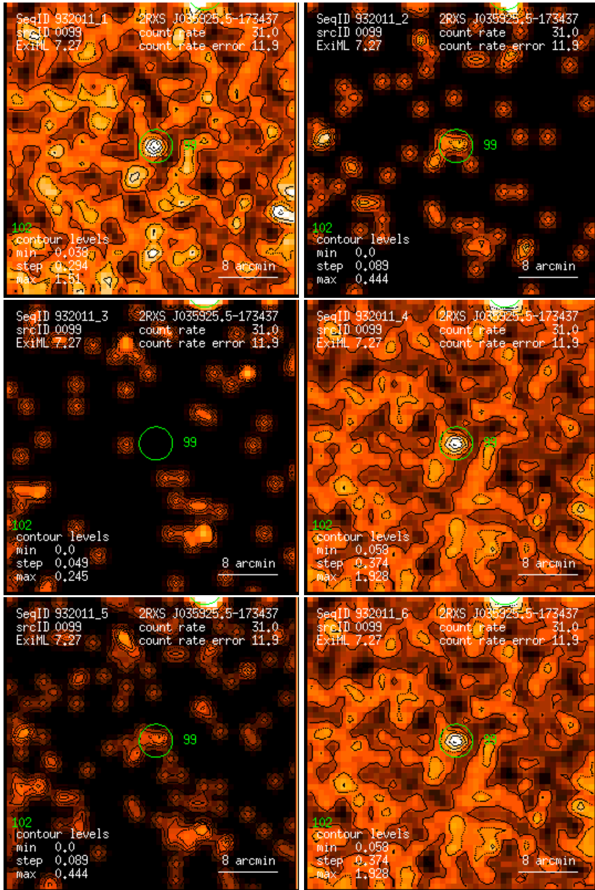
Figure 99: RASS 932011: detection 0099: band rate images, Gaussian filter: (1) PSPC channels 11 – 41, (2) 52 – 90, (3) 91 – 201, (4) 11 – 235, (5) 52 – 201, (6) 11 – 201. Broad band rates in counts/ks. Band rate contour levels in counts/ks/arcmin 2 .
