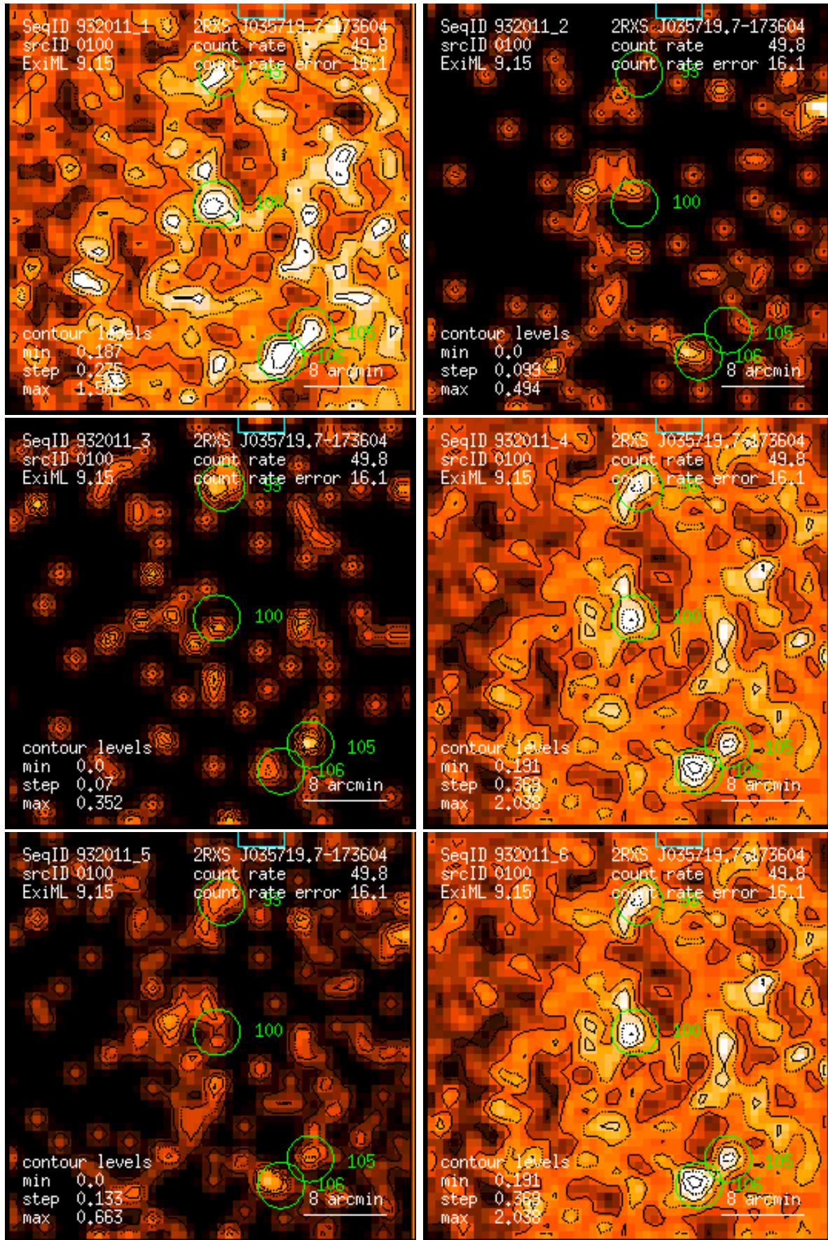
Figure 100: RASS 932011: detection 0100: band rate images, Gaussian filter: (1) PSPC channels 11 – 41, (2) 52 – 90, (3) 91 – 201, (4) 11 – 235, (5) 52 – 201, (6) 11 – 201. Broad band rates in counts/ks. Band rate contour levels in counts/ks/arcmin 2 .
