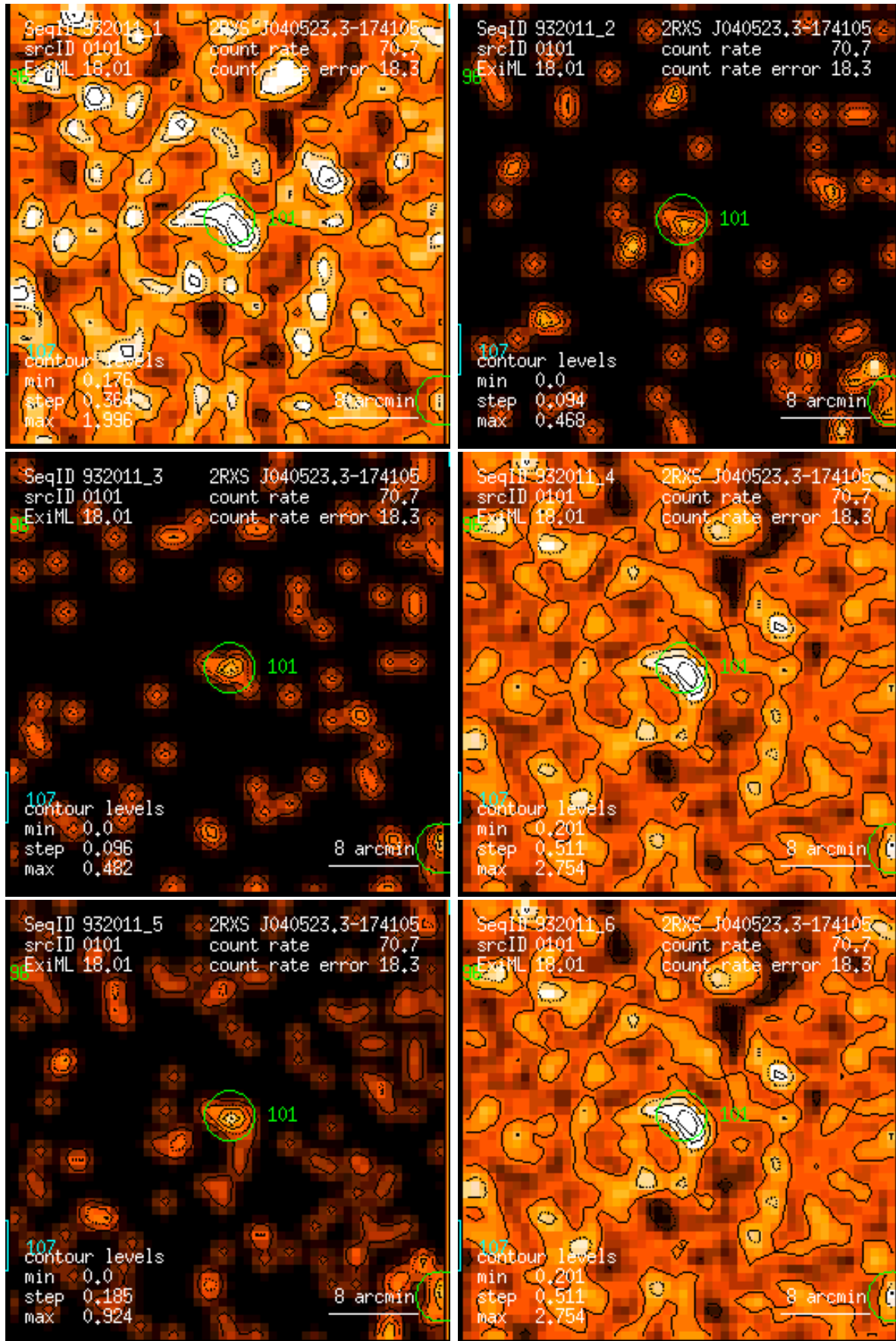
Figure 101: RASS 932011: detection 0101: band rate images, Gaussian filter: (1) PSPC channels 11 – 41, (2) 52 – 90, (3) 91 – 201, (4) 11 – 235, (5) 52 – 201, (6) 11 – 201. Broad band rates in counts/ks. Band rate contour levels in counts/ks/arcmin 2 .
