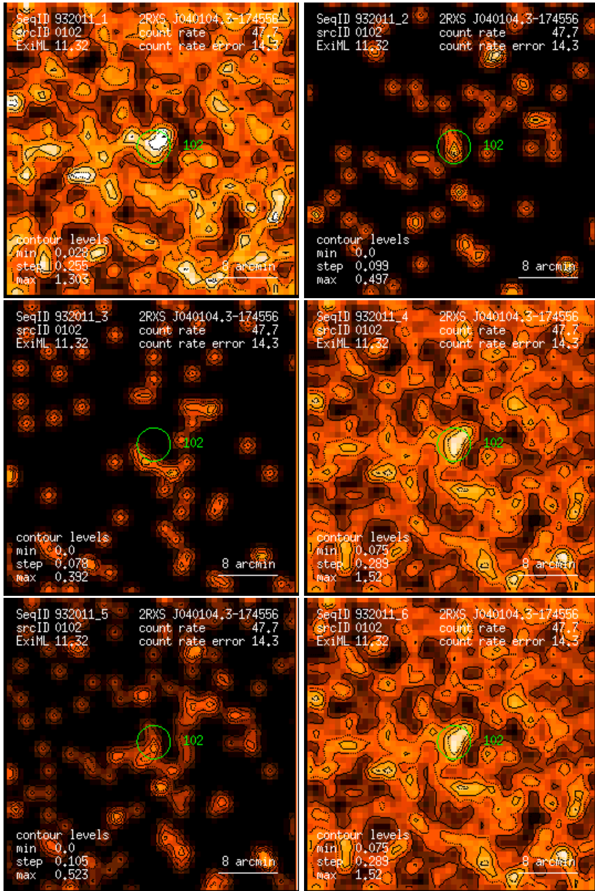
Figure 102: RASS 932011: detection 0102: band rate images, Gaussian filter: (1) PSPC channels 11 – 41, (2) 52 – 90, (3) 91 – 201, (4) 11 – 235, (5) 52 – 201, (6) 11 – 201. Broad band rates in counts/ks. Band rate contour levels in counts/ks/arcmin 2 .
