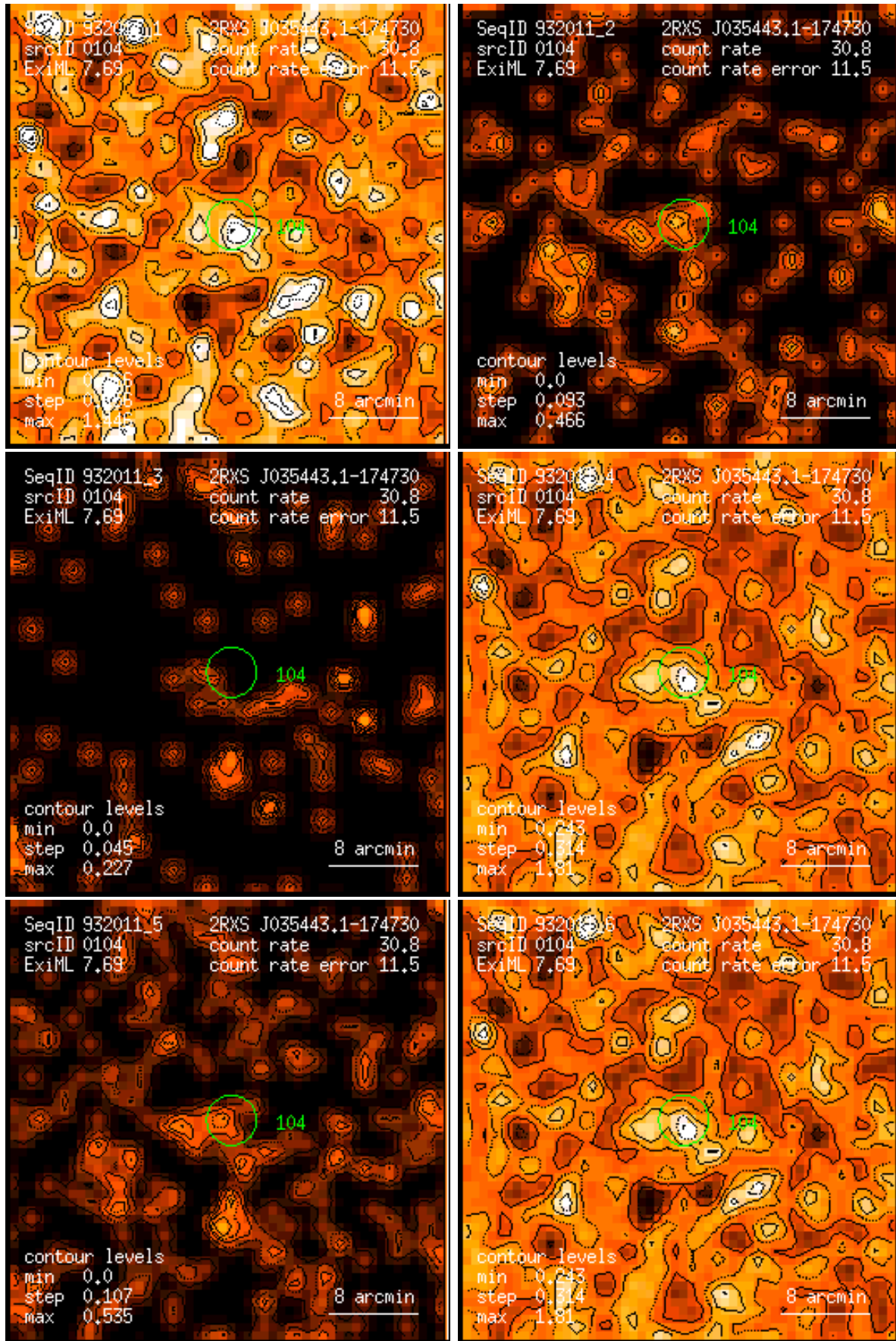
Figure 104: RASS 932011: detection 0104: band rate images, Gaussian filter: (1) PSPC channels 11 – 41, (2) 52 – 90, (3) 91 – 201, (4) 11 – 235, (5) 52 – 201, (6) 11 – 201. Broad band rates in counts/ks. Band rate contour levels in counts/ks/arcmin 2 .
