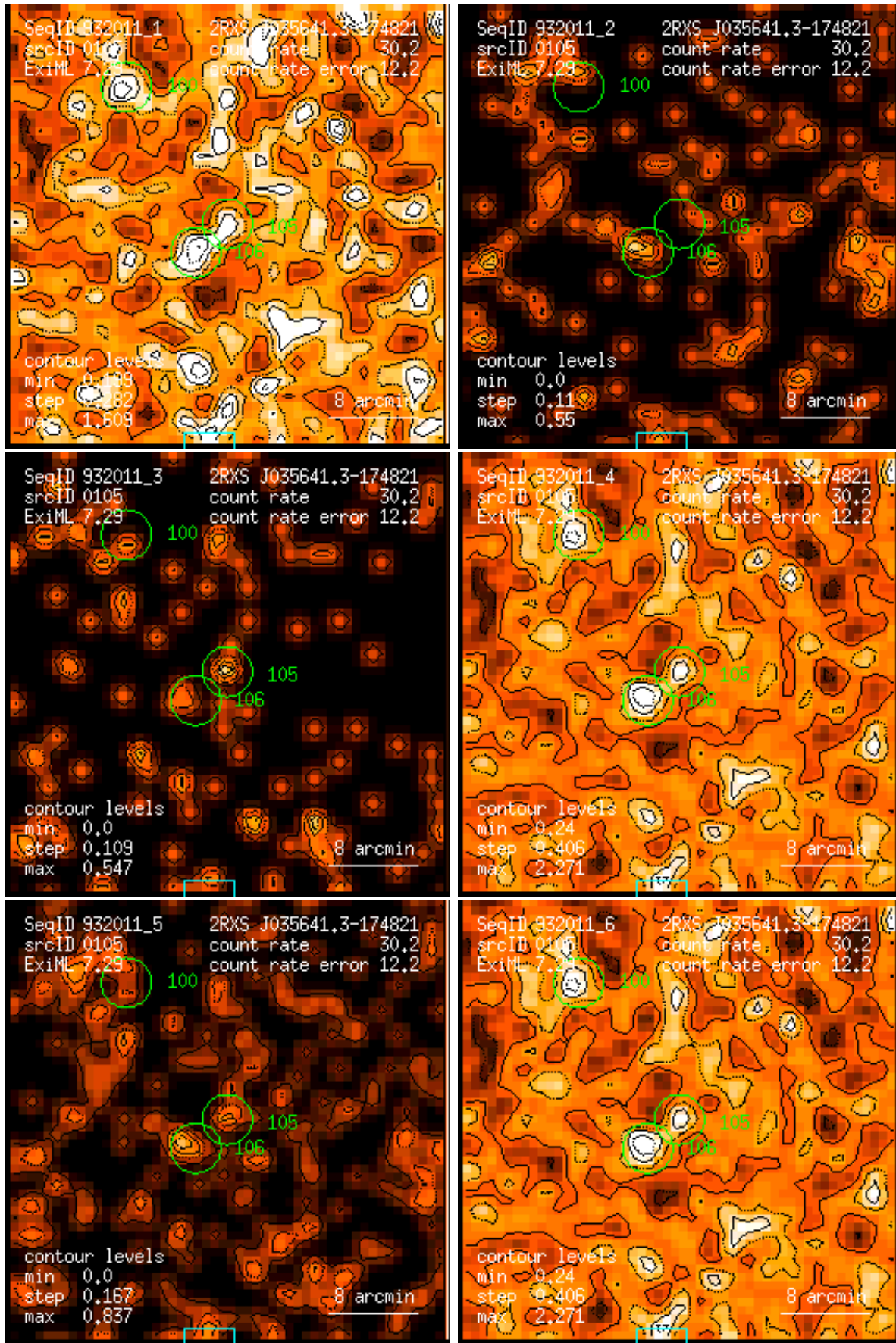
Figure 105: RASS 932011: detection 0105: band rate images, Gaussian filter: (1) PSPC channels 11 – 41, (2) 52 – 90, (3) 91 – 201, (4) 11 – 235, (5) 52 – 201, (6) 11 – 201. Broad band rates in counts/ks. Band rate contour levels in counts/ks/arcmin 2 .
