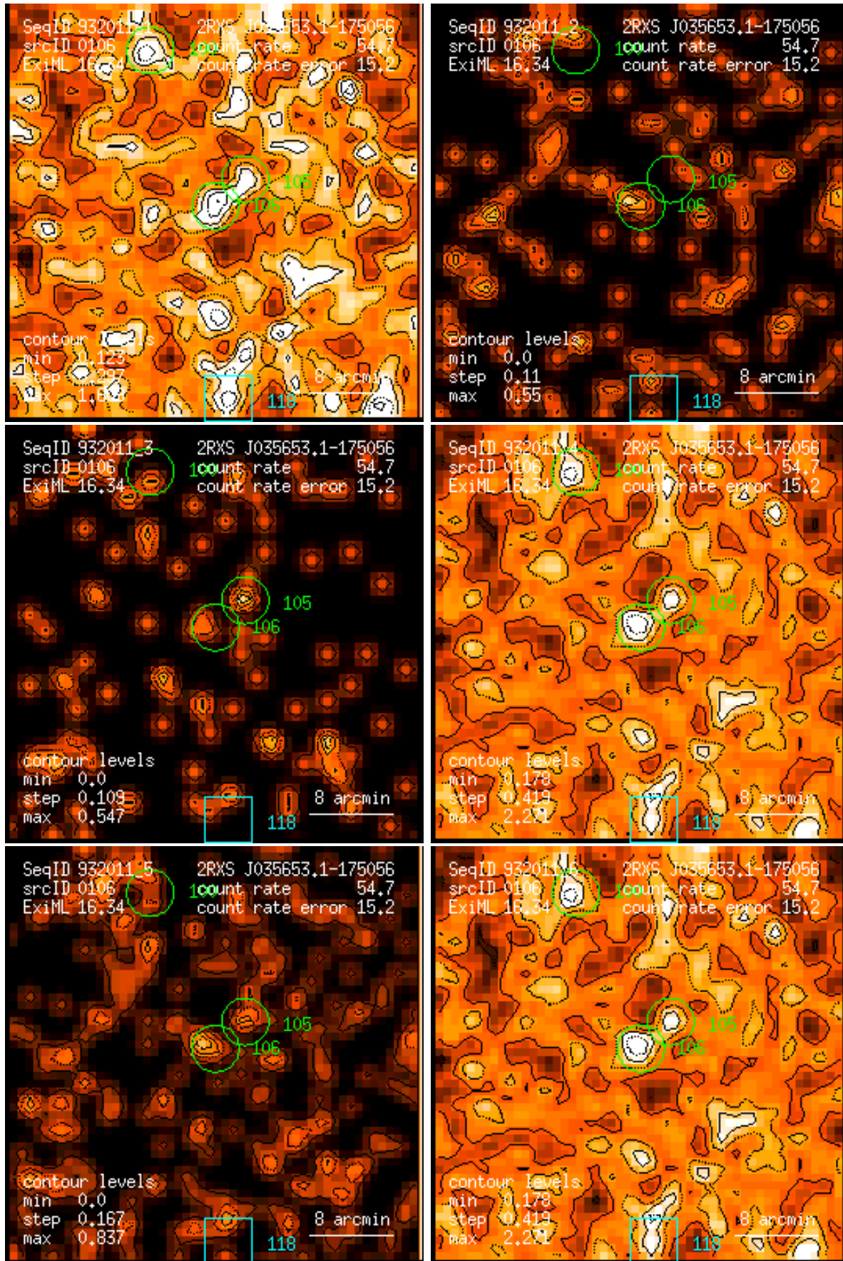
Figure 106: RASS 932011: detection 0106: band rate images, Gaussian filter: (1) PSPC channels 11 – 41, (2) 52 – 90, (3) 91 – 201, (4) 11 – 235, (5) 52 – 201, (6) 11 – 201. Broad band rates in counts/ks. Band rate contour levels in counts/ks/arcmin 2 .
