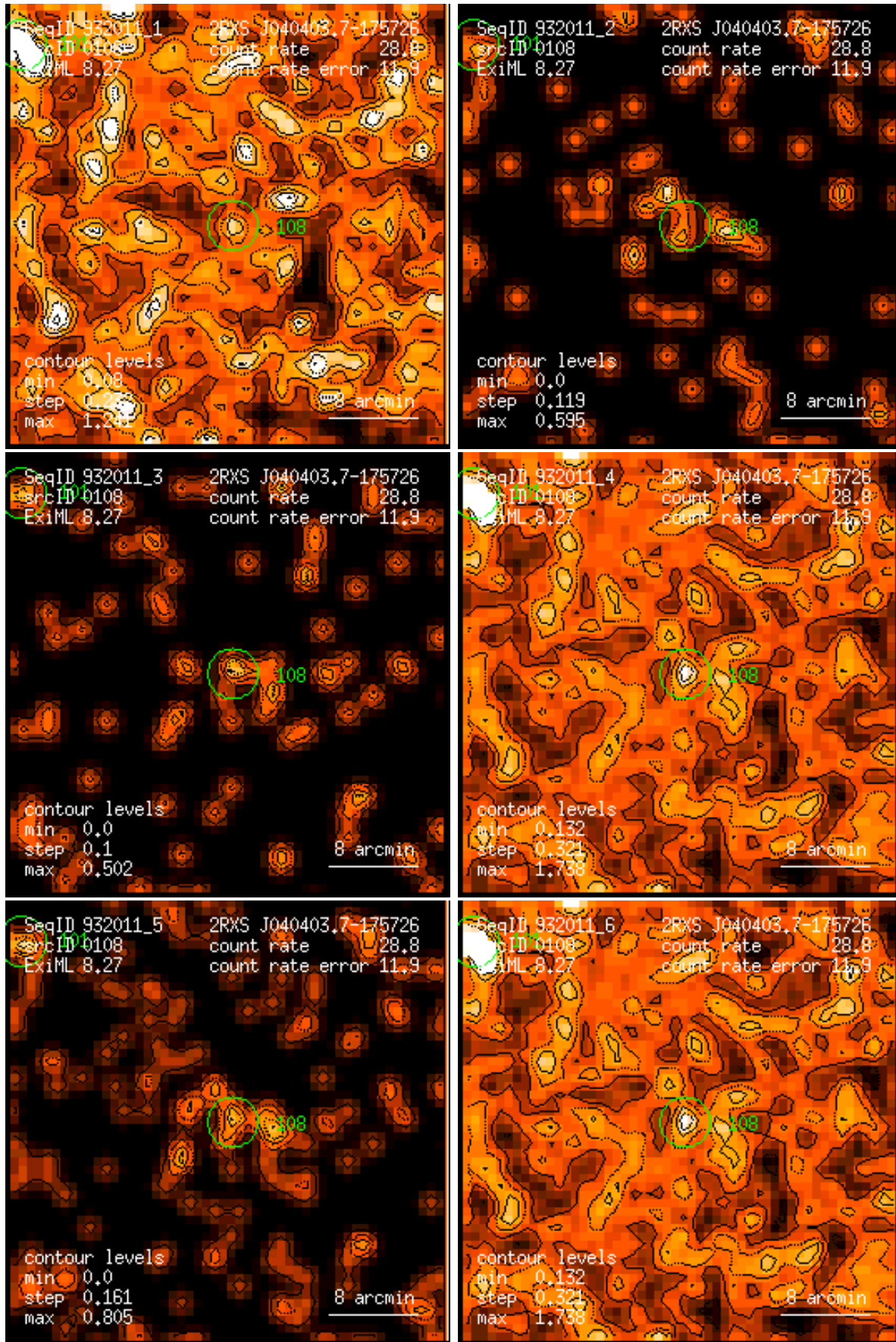
Figure 108: RASS 932011: detection 0108: band rate images, Gaussian filter: (1) PSPC channels 11 – 41, (2) 52 – 90, (3) 91 – 201, (4) 11 – 235, (5) 52 – 201, (6) 11 – 201. Broad band rates in counts/ks. Band rate contour levels in counts/ks/arcmin 2 .
