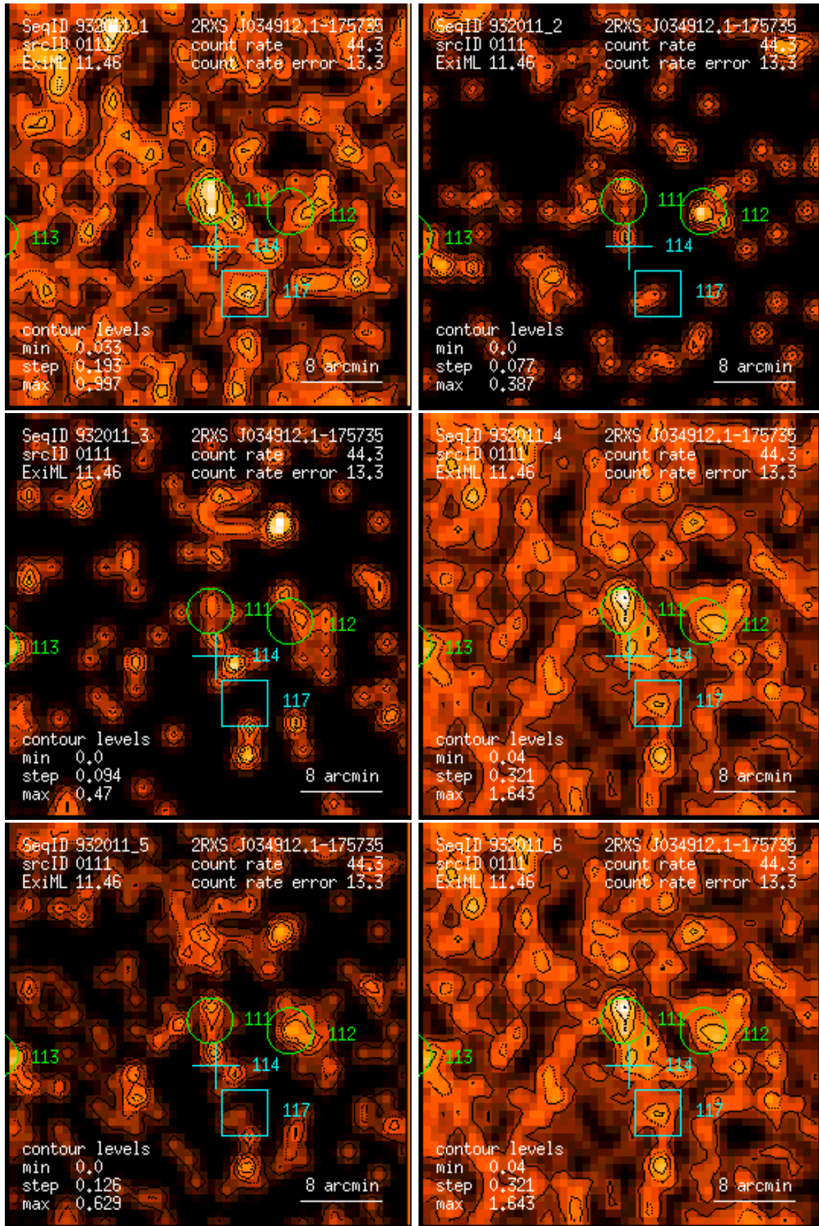
Figure 111: RASS 932011: detection 0111: band rate images, Gaussian filter: (1) PSPC channels 11 – 41, (2) 52 – 90, (3) 91 – 201, (4) 11 – 235, (5) 52 – 201, (6) 11 – 201. Broad band rates in counts/ks. Band rate contour levels in counts/ks/arcmin 2 .
