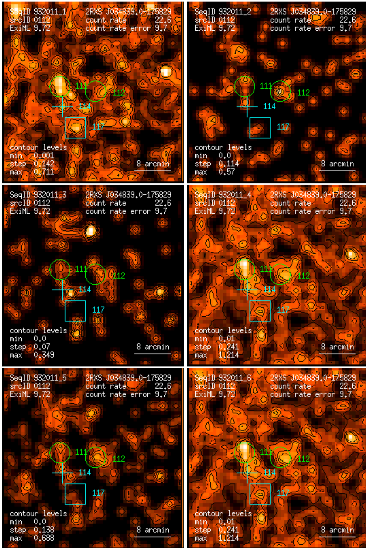
Figure 112: RASS 932011: detection 0112: band rate images, Gaussian filter: (1) PSPC channels 11 – 41, (2) 52 – 90, (3) 91 – 201, (4) 11 – 235, (5) 52 – 201, (6) 11 – 201. Broad band rates in counts/ks. Band rate contour levels in counts/ks/arcmin 2 .
