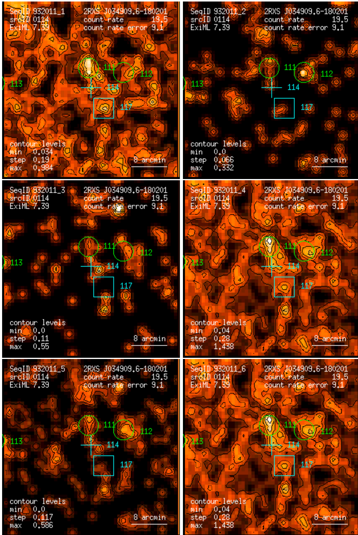
Figure 114: RASS 932011: detection 0114: band rate images, Gaussian filter: (1) PSPC channels 11 – 41, (2) 52 – 90, (3) 91 – 201, (4) 11 – 235, (5) 52 – 201, (6) 11 – 201. Broad band rates in counts/ks. Band rate contour levels in counts/ks/arcmin 2 .
