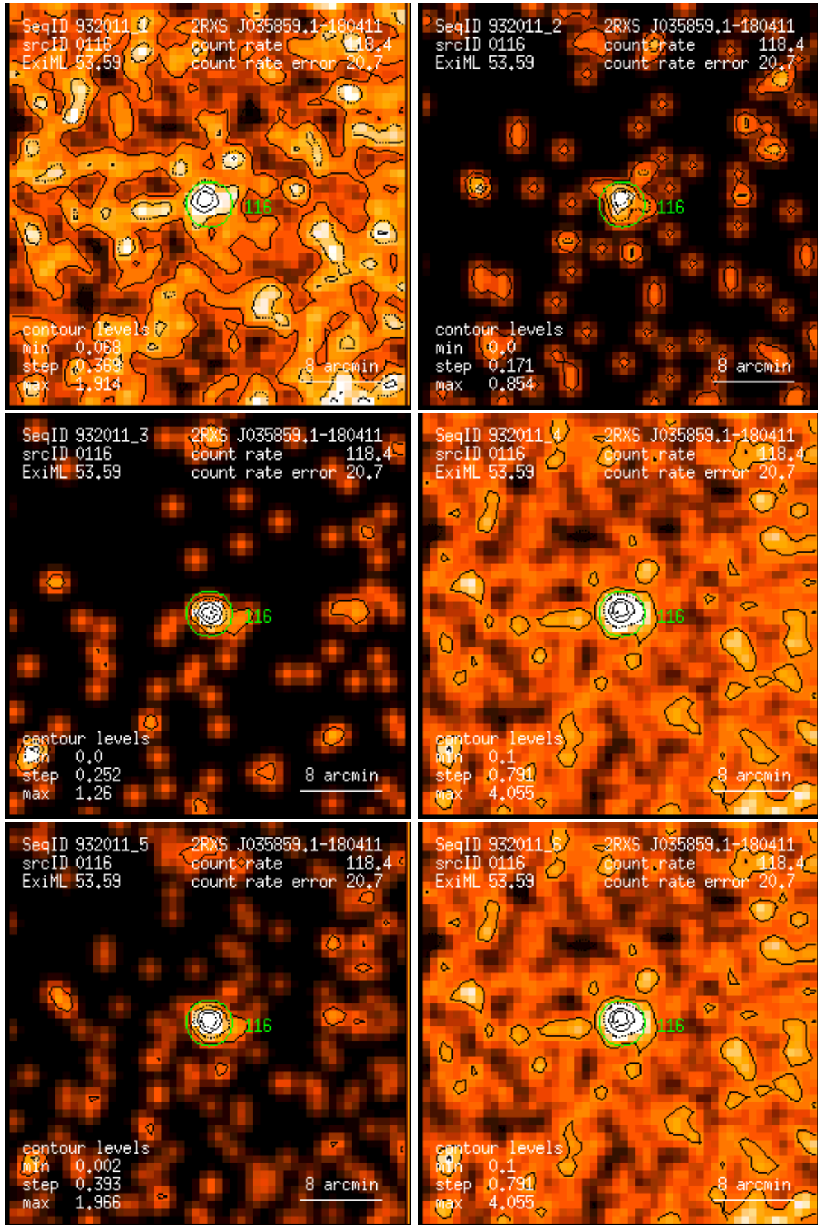
Figure 116: RASS 932011: detection 0116: band rate images, Gaussian filter: (1) PSPC channels 11 – 41, (2) 52 – 90, (3) 91 – 201, (4) 11 – 235, (5) 52 – 201, (6) 11 – 201. Broad band rates in counts/ks. Band rate contour levels in counts/ks/arcmin 2 .
