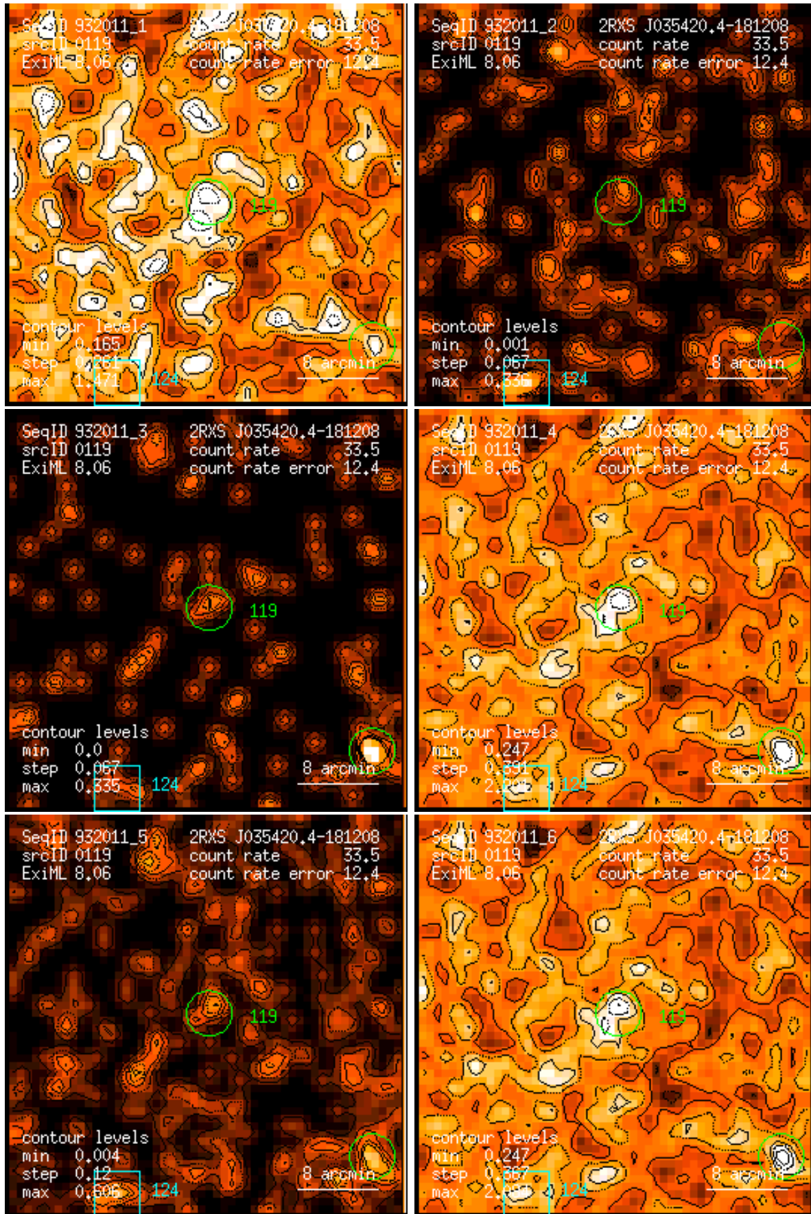
Figure 119: RASS 932011: detection 0119: band rate images, Gaussian filter: (1) PSPC channels 11 – 41, (2) 52 – 90, (3) 91 – 201, (4) 11 – 235, (5) 52 – 201, (6) 11 – 201. Broad band rates in counts/ks. Band rate contour levels in counts/ks/arcmin 2 .
