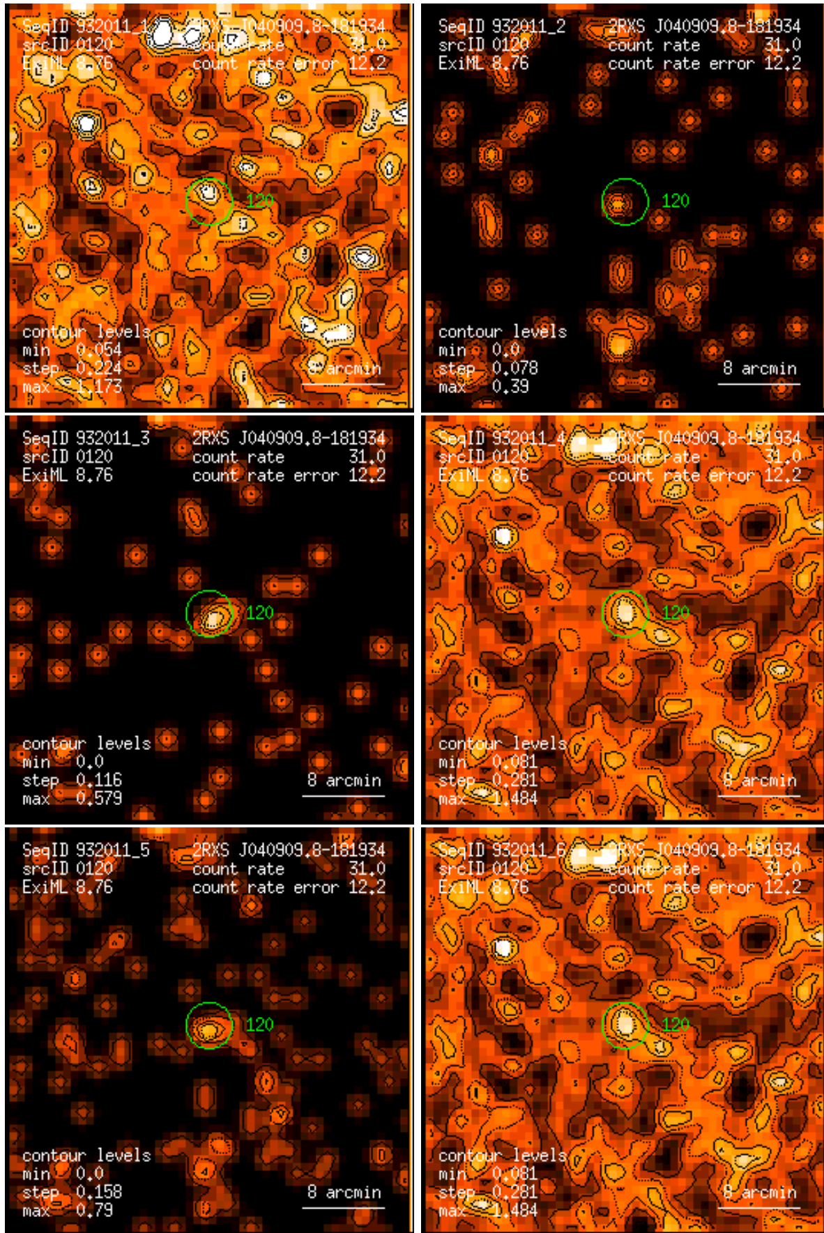
Figure 120: RASS 932011: detection 0120: band rate images, Gaussian filter: (1) PSPC channels 11 – 41, (2) 52 – 90, (3) 91 – 201, (4) 11 – 235, (5) 52 – 201, (6) 11 – 201. Broad band rates in counts/ks. Band rate contour levels in counts/ks/arcmin 2 .
