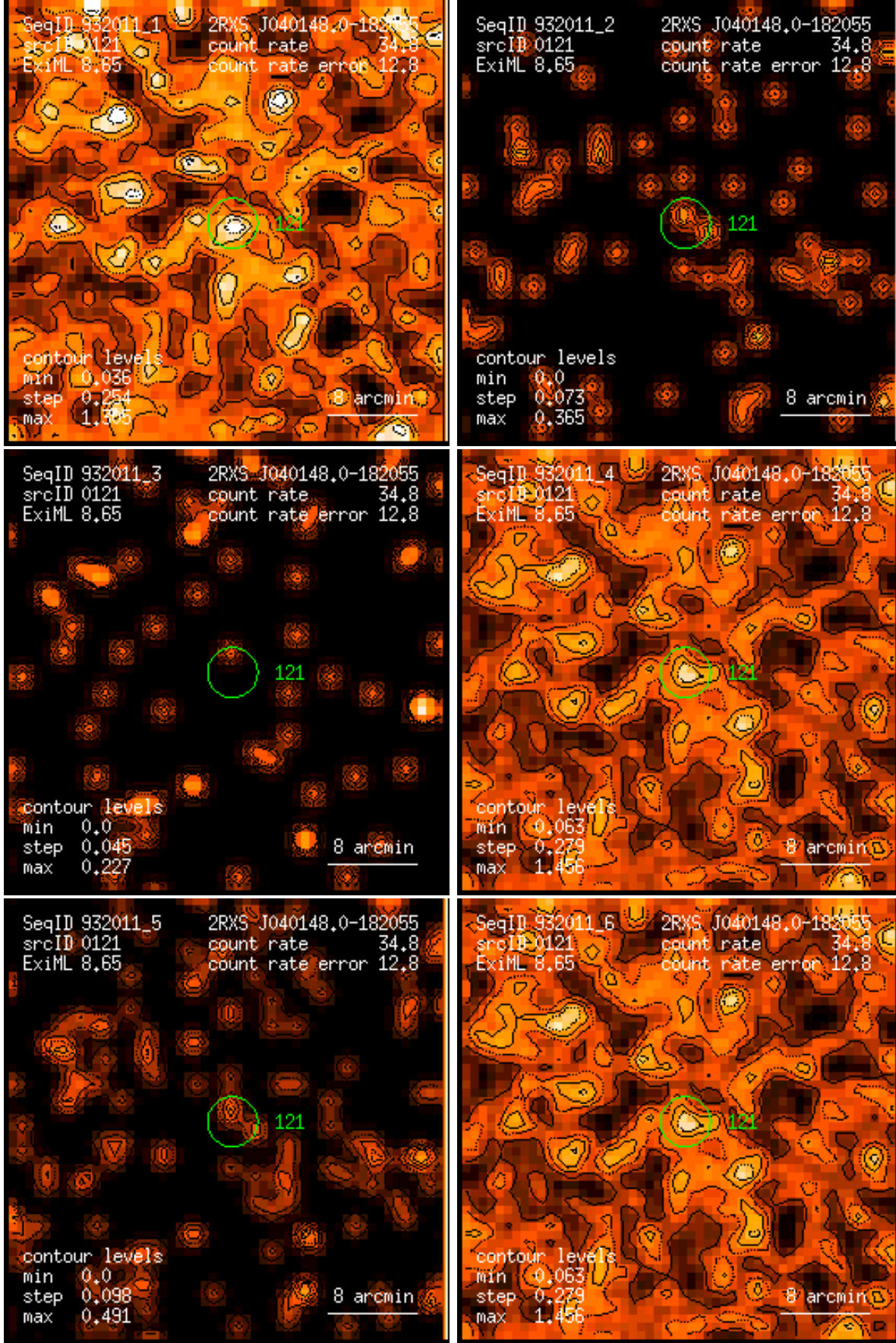
Figure 121: RASS 932011: detection 0121: band rate images, Gaussian filter: (1) PSPC channels 11 – 41, (2) 52 – 90, (3) 91 – 201, (4) 11 – 235, (5) 52 – 201, (6) 11 – 201. Broad band rates in counts/ks. Band rate contour levels in counts/ks/arcmin 2 .
