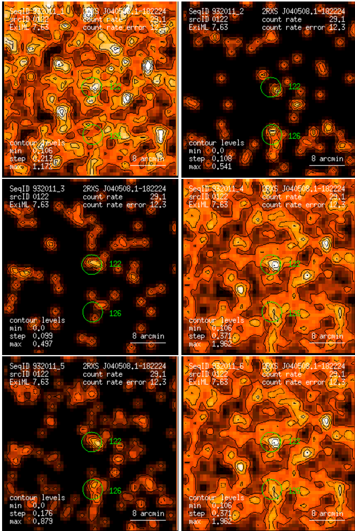
Figure 122: RASS 932011: detection 0122: band rate images, Gaussian filter: (1) PSPC channels 11 – 41, (2) 52 – 90, (3) 91 – 201, (4) 11 – 235, (5) 52 – 201, (6) 11 – 201. Broad band rates in counts/ks. Band rate contour levels in counts/ks/arcmin 2 .
