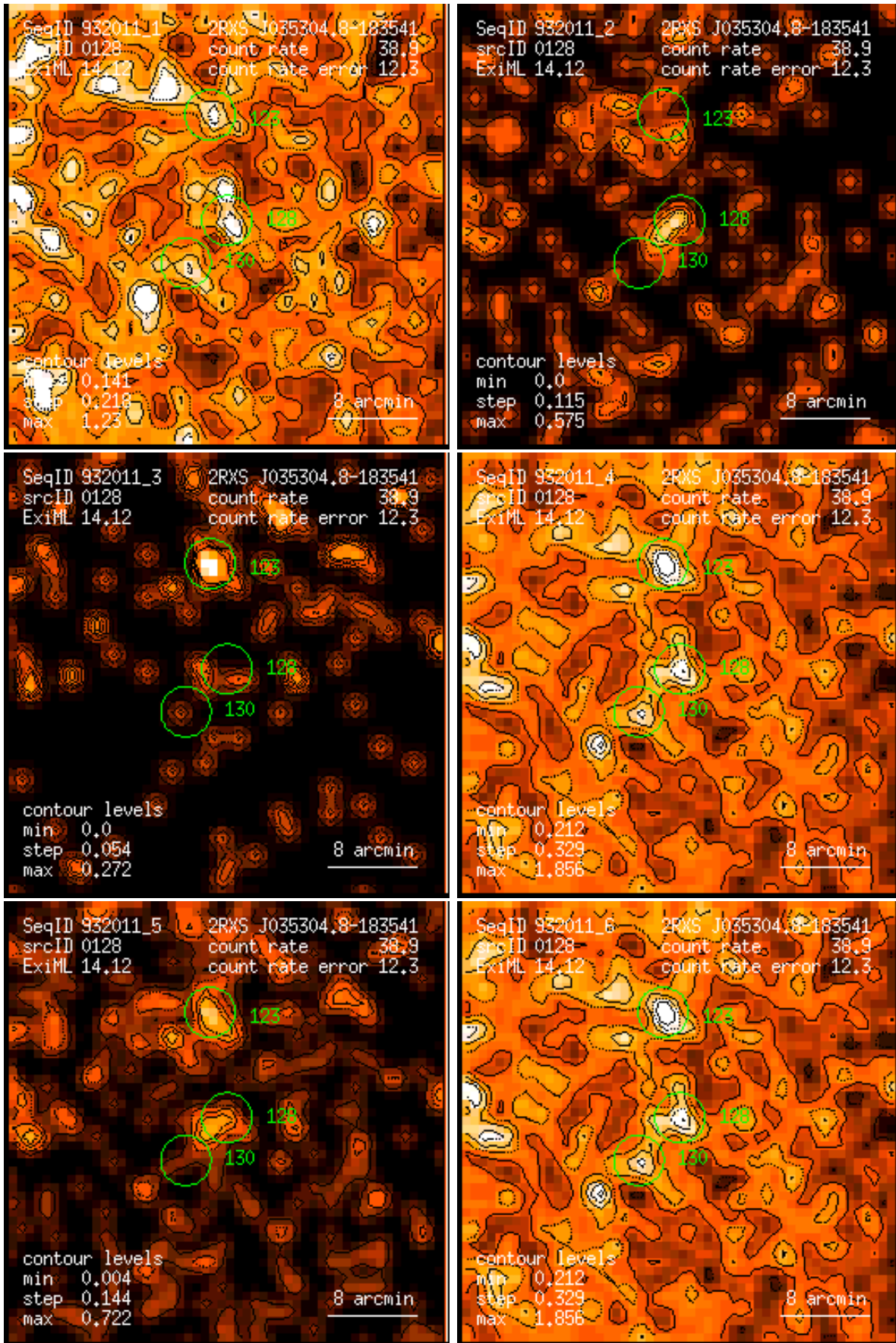
Figure 128: RASS 932011: detection 0128: band rate images, Gaussian filter: (1) PSPC channels 11 – 41, (2) 52 – 90, (3) 91 – 201, (4) 11 – 235, (5) 52 – 201, (6) 11 – 201. Broad band rates in counts/ks. Band rate contour levels in counts/ks/arcmin 2 .
