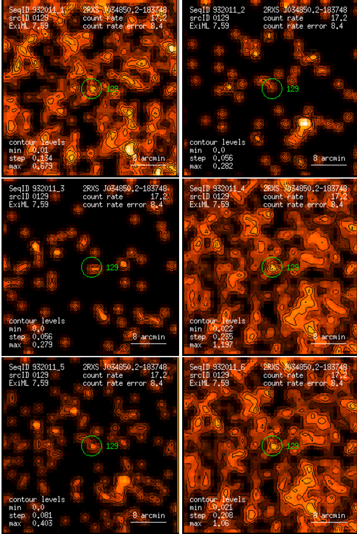
Figure 129: RASS 932011: detection 0129: band rate images, Gaussian filter: (1) PSPC channels 11 – 41, (2) 52 – 90, (3) 91 – 201, (4) 11 – 235, (5) 52 – 201, (6) 11 – 201. Broad band rates in counts/ks. Band rate contour levels in counts/ks/arcmin 2 .
