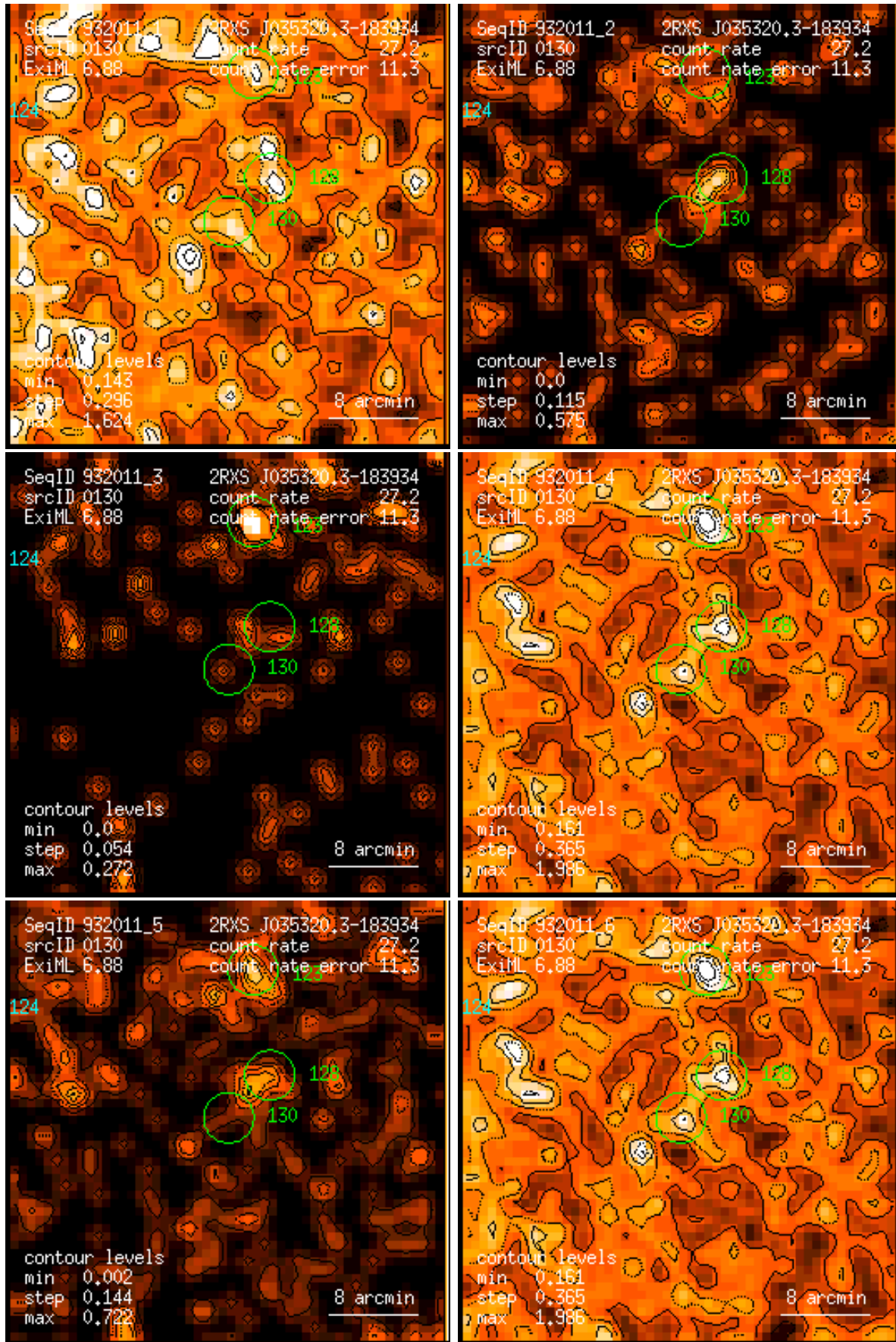
Figure 130: RASS 932011: detection 0130: band rate images, Gaussian filter: (1) PSPC channels 11 – 41, (2) 52 – 90, (3) 91 – 201, (4) 11 – 235, (5) 52 – 201, (6) 11 – 201. Broad band rates in counts/ks. Band rate contour levels in counts/ks/arcmin 2 .
