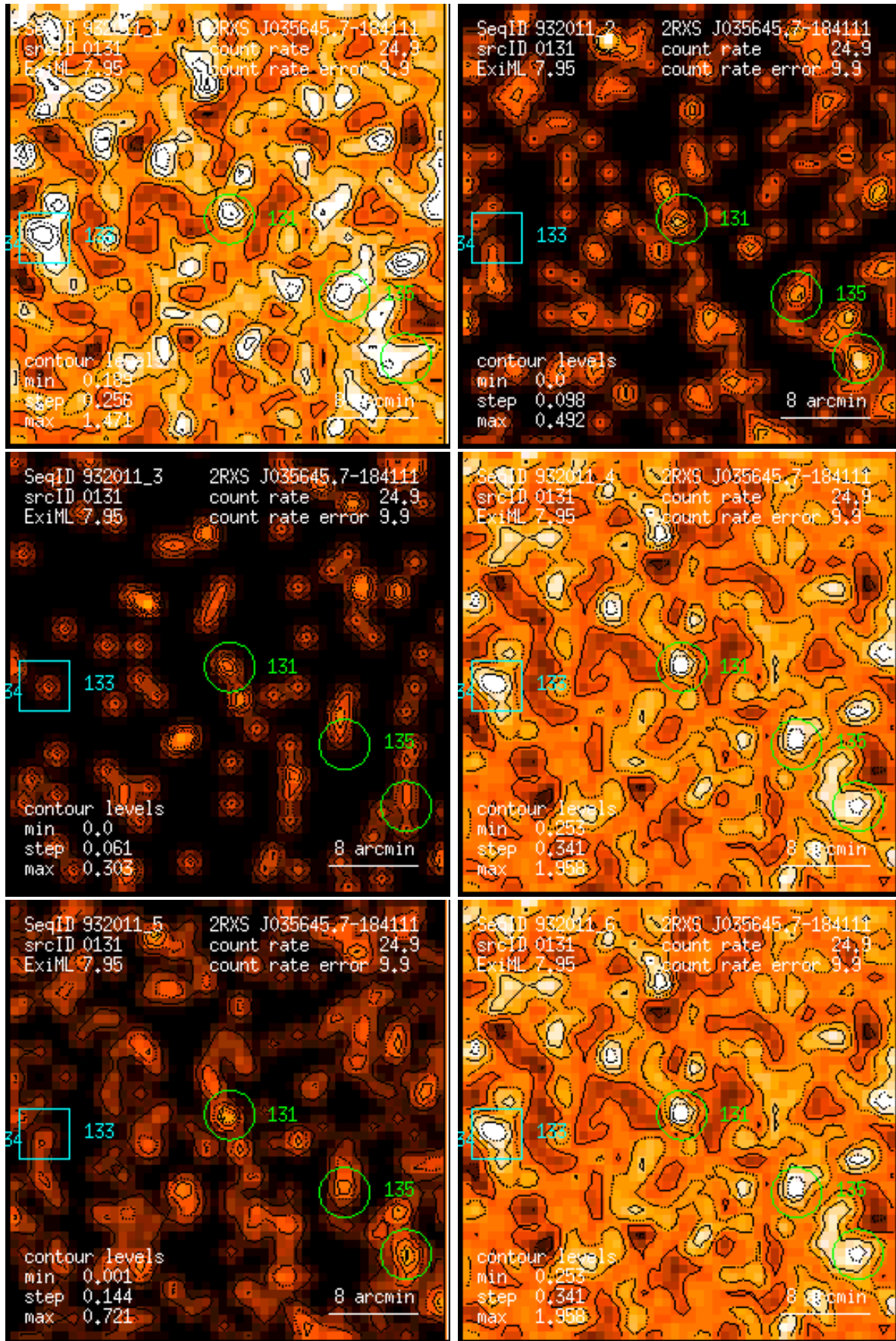
Figure 131: RASS 932011: detection 0131: band rate images, Gaussian filter: (1) PSPC channels 11 – 41, (2) 52 – 90, (3) 91 – 201, (4) 11 – 235, (5) 52 – 201, (6) 11 – 201. Broad band rates in counts/ks. Band rate contour levels in counts/ks/arcmin 2 .
