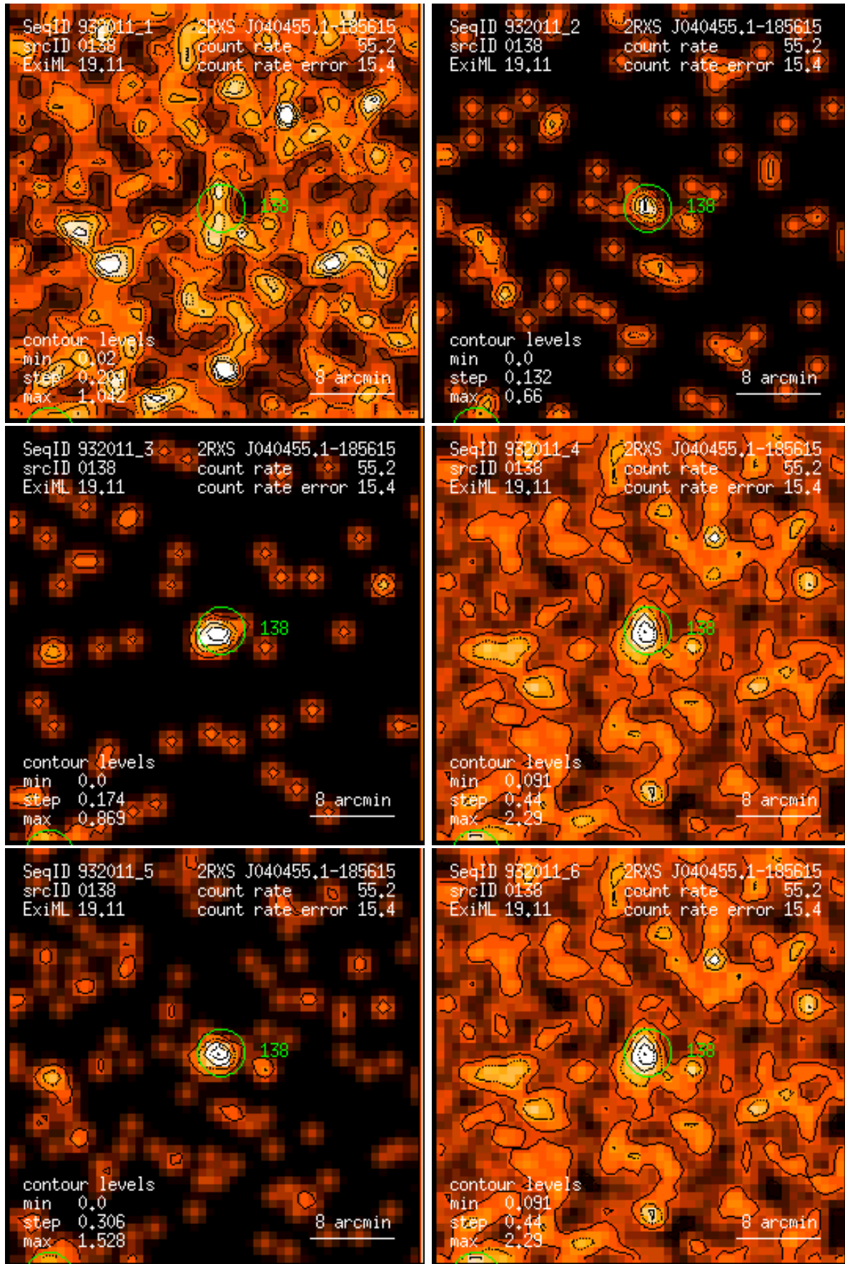
Figure 138: RASS 932011: detection 0138: band rate images, Gaussian filter: (1) PSPC channels 11 – 41, (2) 52 – 90, (3) 91 – 201, (4) 11 – 235, (5) 52 – 201, (6) 11 – 201. Broad band rates in counts/ks. Band rate contour levels in counts/ks/arcmin 2 .
