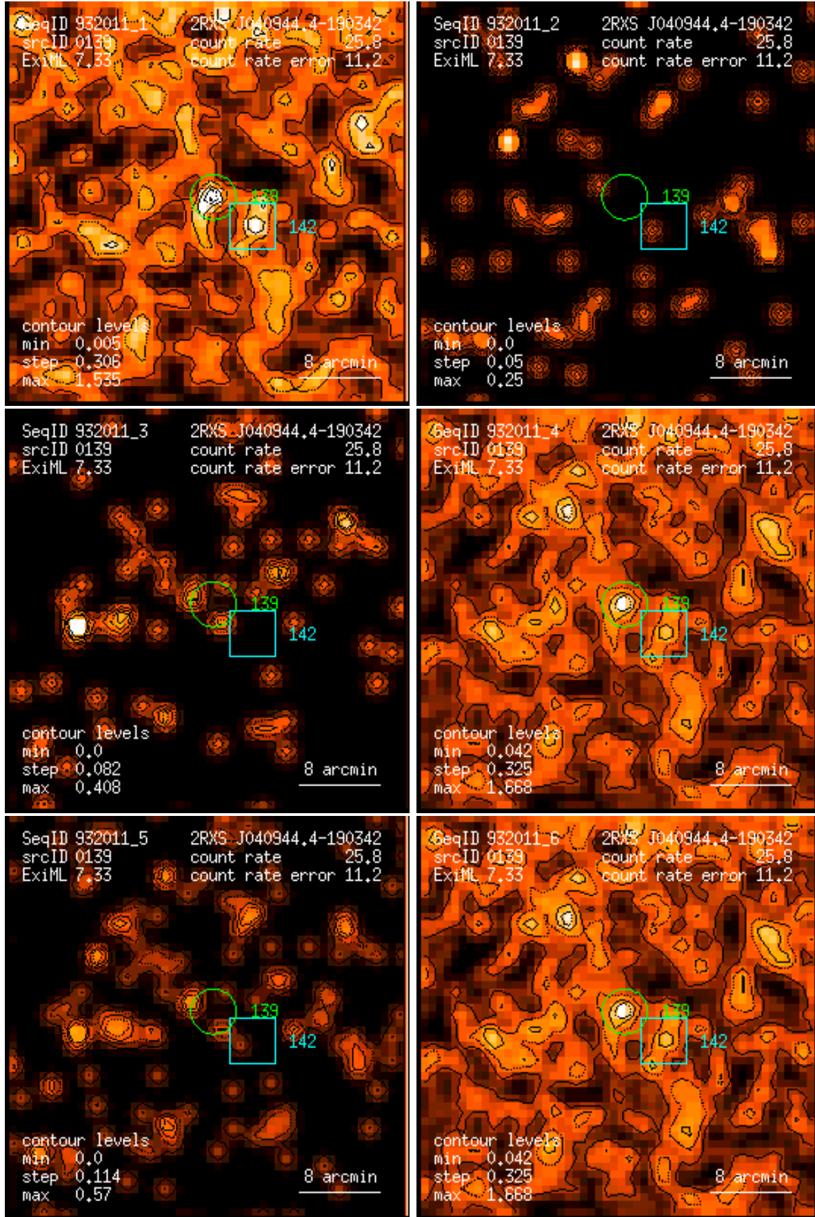
Figure 139: RASS 932011: detection 0139: band rate images, Gaussian filter: (1) PSPC channels 11 – 41, (2) 52 – 90, (3) 91 – 201, (4) 11 – 235, (5) 52 – 201, (6) 11 – 201. Broad band rates in counts/ks. Band rate contour levels in counts/ks/arcmin 2 .
