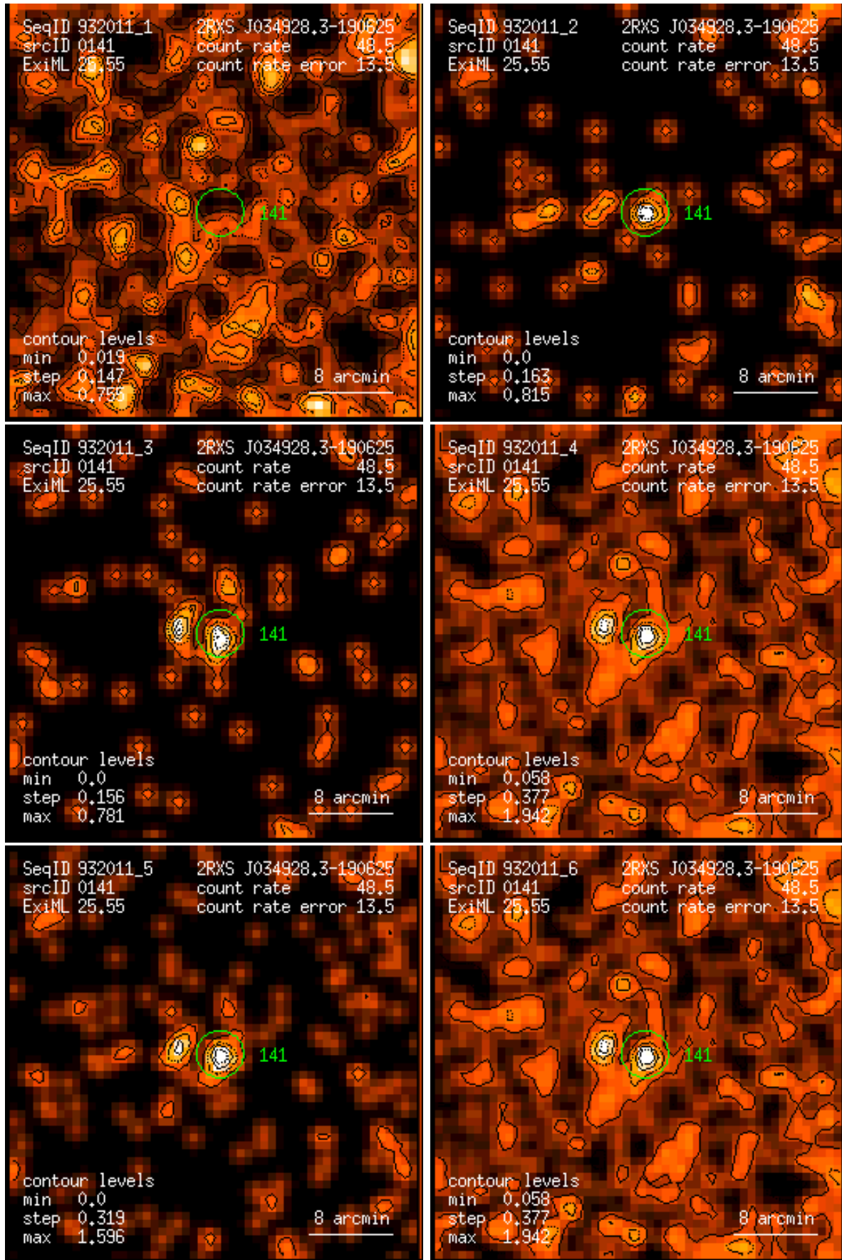
Figure 141: RASS 932011: detection 0141: band rate images, Gaussian filter: (1) PSPC channels 11 – 41, (2) 52 – 90, (3) 91 – 201, (4) 11 – 235, (5) 52 – 201, (6) 11 – 201. Broad band rates in counts/ks. Band rate contour levels in counts/ks/arcmin 2 .
