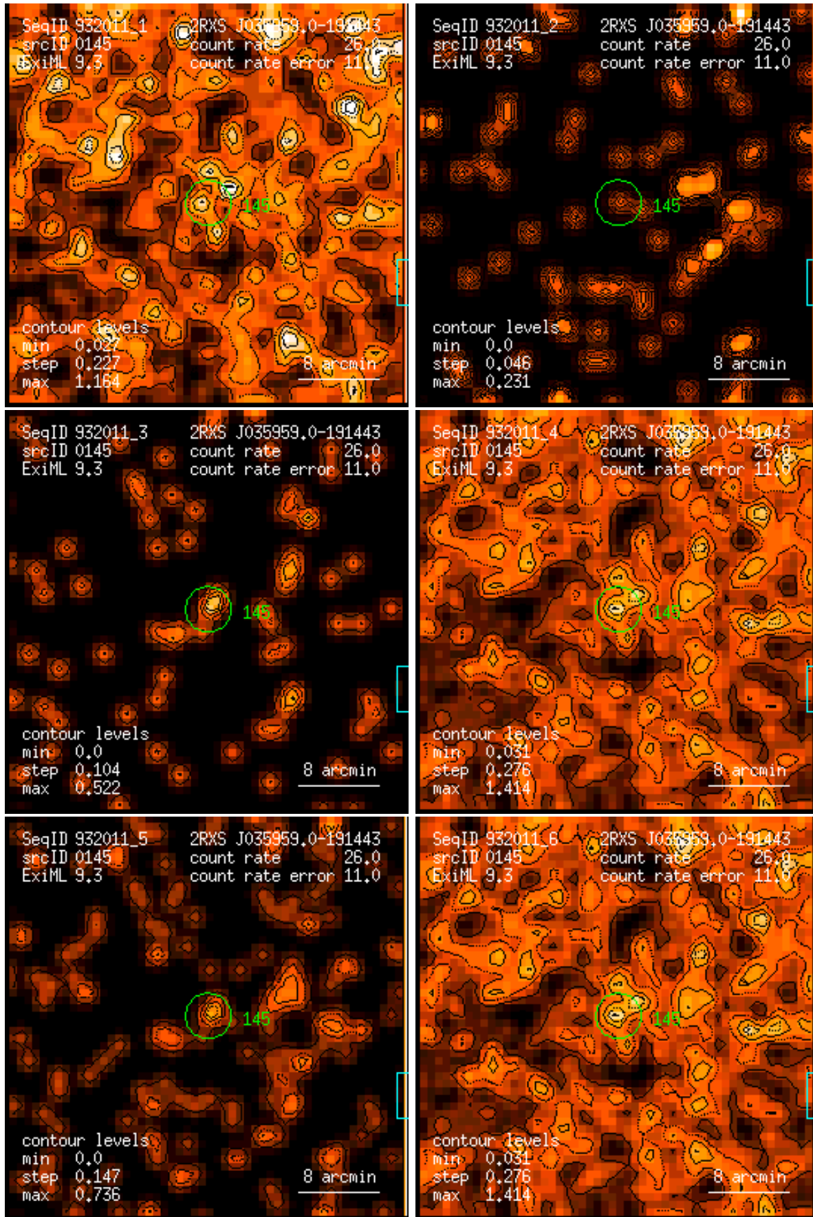
Figure 145: RASS 932011: detection 0145: band rate images, Gaussian filter: (1) PSPC channels 11 – 41, (2) 52 – 90, (3) 91 – 201, (4) 11 – 235, (5) 52 – 201, (6) 11 – 201. Broad band rates in counts/ks. Band rate contour levels in counts/ks/arcmin 2 .
