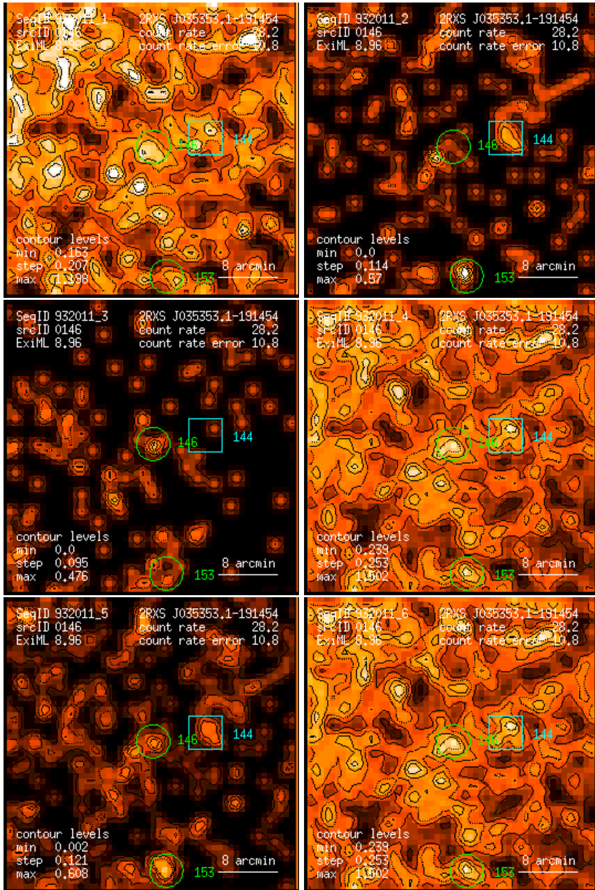
Figure 146: RASS 932011: detection 0146: band rate images, Gaussian filter: (1) PSPC channels 11 – 41, (2) 52 – 90, (3) 91 – 201, (4) 11 – 235, (5) 52 – 201, (6) 11 – 201. Broad band rates in counts/ks. Band rate contour levels in counts/ks/arcmin 2 .
