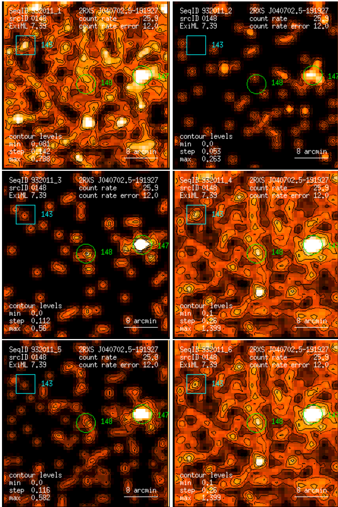
Figure 148: RASS 932011: detection 0148: band rate images, Gaussian filter: (1) PSPC channels 11 – 41, (2) 52 – 90, (3) 91 – 201, (4) 11 – 235, (5) 52 – 201, (6) 11 – 201. Broad band rates in counts/ks. Band rate contour levels in counts/ks/arcmin 2 .
