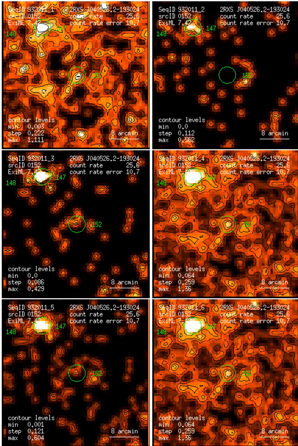
Figure 152: RASS 932011: detection 0152: band rate images, Gaussian filter: (1) PSPC channels 11 – 41, (2) 52 – 90, (3) 91 – 201, (4) 11 – 235, (5) 52 – 201, (6) 11 – 201. Broad band rates in counts/ks. Band rate contour levels in counts/ks/arcmin 2 .
