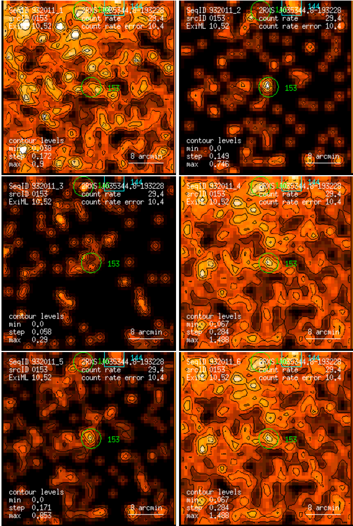
Figure 153: RASS 932011: detection 0153: band rate images, Gaussian filter: (1) PSPC channels 11 – 41, (2) 52 – 90, (3) 91 – 201, (4) 11 – 235, (5) 52 – 201, (6) 11 – 201. Broad band rates in counts/ks. Band rate contour levels in counts/ks/arcmin 2 .
