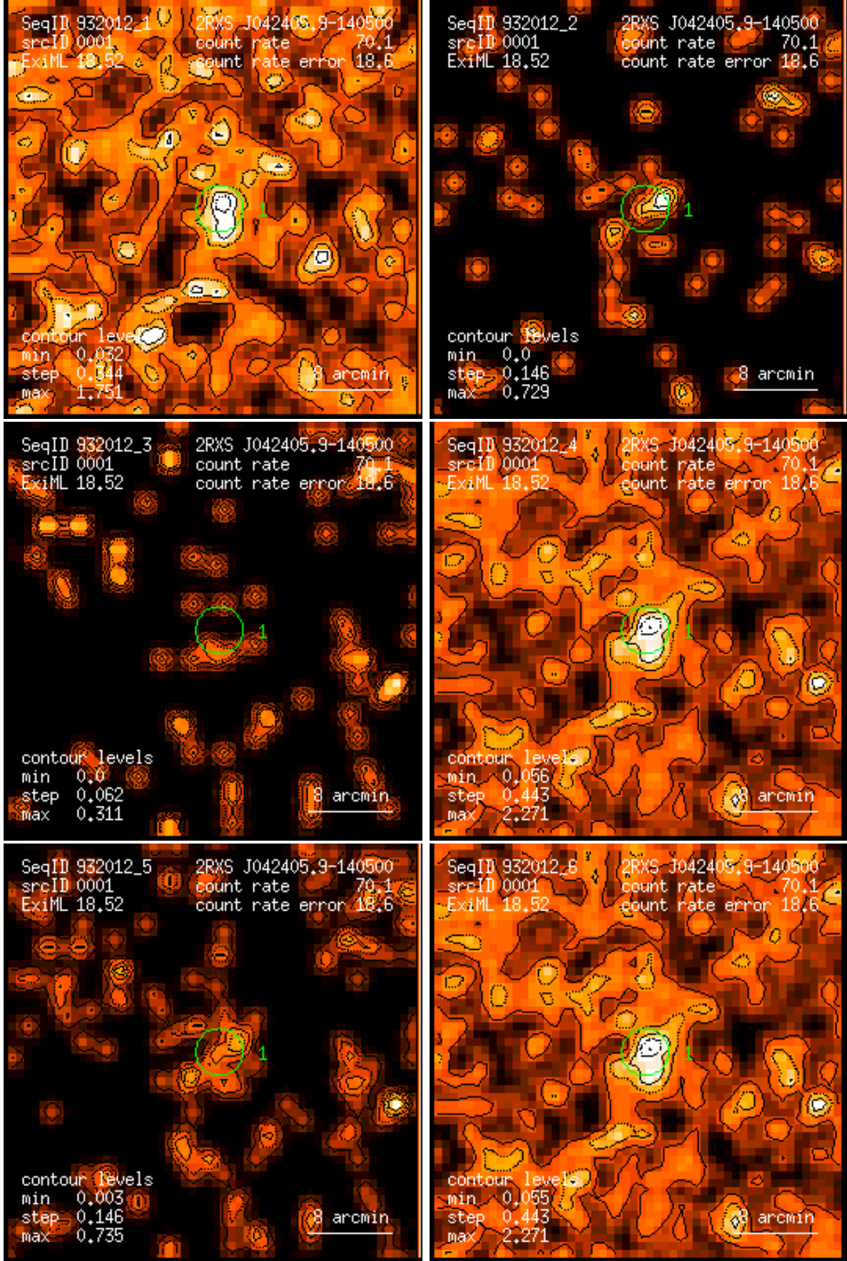
Figure 1: RASS 932012: detection 0001: band rate images, Gaussian filter: (1) PSPC channels 11 – 41, (2) 52 – 90, (3) 91 – 201, (4) 11 – 235, (5) 52 – 201, (6) 11 – 201. Broad band rates in counts/ks. Band rate contour levels in counts/ks/arcmin 2 .
