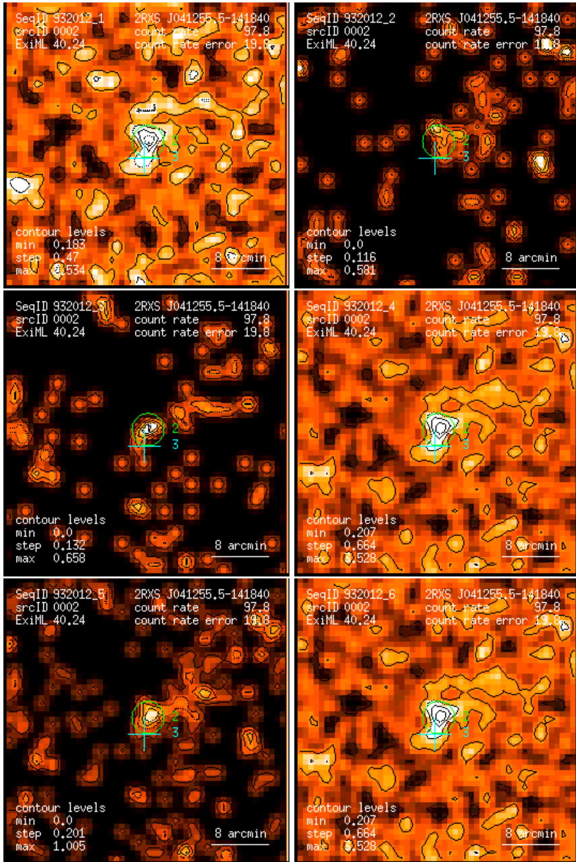
Figure 2: RASS 932012: detection 0002: band rate images, Gaussian filter: (1) PSPC channels 11 – 41, (2) 52 – 90, (3) 91 – 201, (4) 11 – 235, (5) 52 – 201, (6) 11 – 201. Broad band rates in counts/ks. Band rate contour levels in counts/ks/arcmin 2 .
