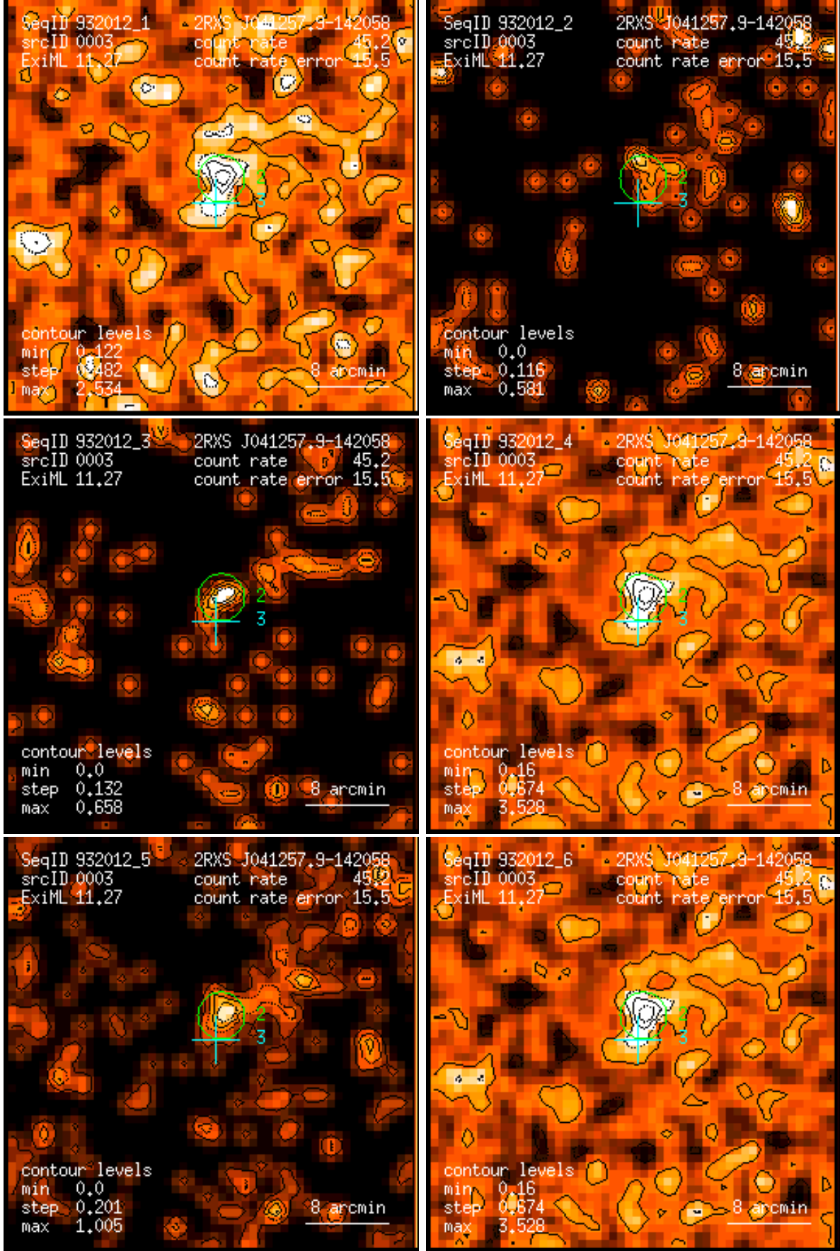
Figure 3: RASS 932012: detection 0003: band rate images, Gaussian filter: (1) PSPC channels 11 – 41, (2) 52 – 90, (3) 91 – 201, (4) 11 – 235, (5) 52 – 201, (6) 11 – 201. Broad band rates in counts/ks. Band rate contour levels in counts/ks/arcmin 2 .
