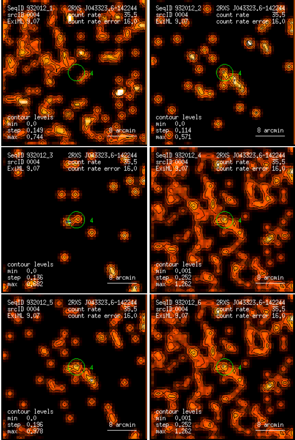
Figure 4: RASS 932012: detection 0004: band rate images, Gaussian filter: (1) PSPC channels 11 – 41, (2) 52 – 90, (3) 91 – 201, (4) 11 – 235, (5) 52 – 201, (6) 11 – 201. Broad band rates in counts/ks. Band rate contour levels in counts/ks/arcmin 2 .
