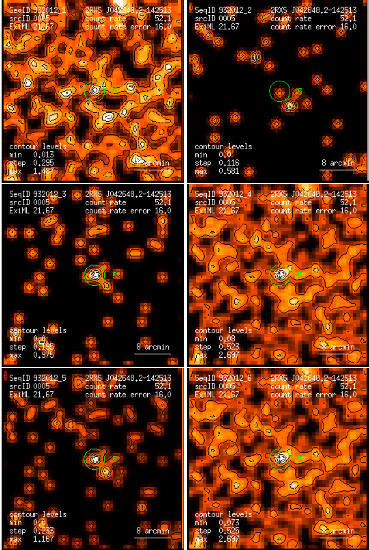
Figure 5: RASS 932012: detection 0005: band rate images, Gaussian filter: (1) PSPC channels 11 – 41, (2) 52 – 90, (3) 91 – 201, (4) 11 – 235, (5) 52 – 201, (6) 11 – 201. Broad band rates in counts/ks. Band rate contour levels in counts/ks/arcmin 2 .
