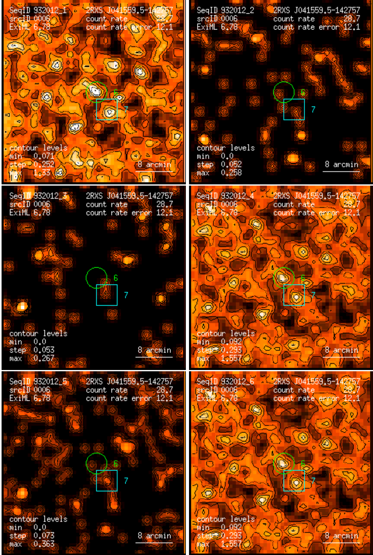
Figure 6: RASS 932012: detection 0006: band rate images, Gaussian filter: (1) PSPC channels 11 – 41, (2) 52 – 90, (3) 91 – 201, (4) 11 – 235, (5) 52 – 201, (6) 11 – 201. Broad band rates in counts/ks. Band rate contour levels in counts/ks/arcmin 2 .
