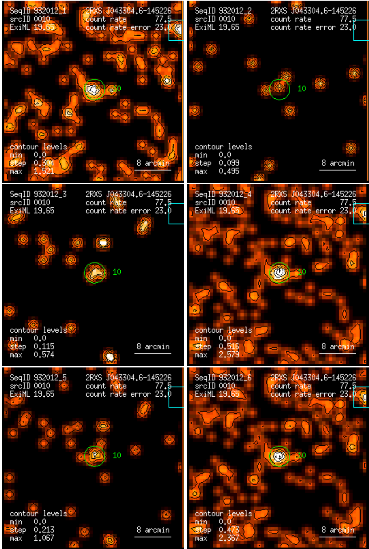
Figure 10: RASS 932012: detection 0010: band rate images, Gaussian filter: (1) PSPC channels 11 – 41, (2) 52 – 90, (3) 91 – 201, (4) 11 – 235, (5) 52 – 201, (6) 11 – 201. Broad band rates in counts/ks. Band rate contour levels in counts/ks/arcmin 2 .
