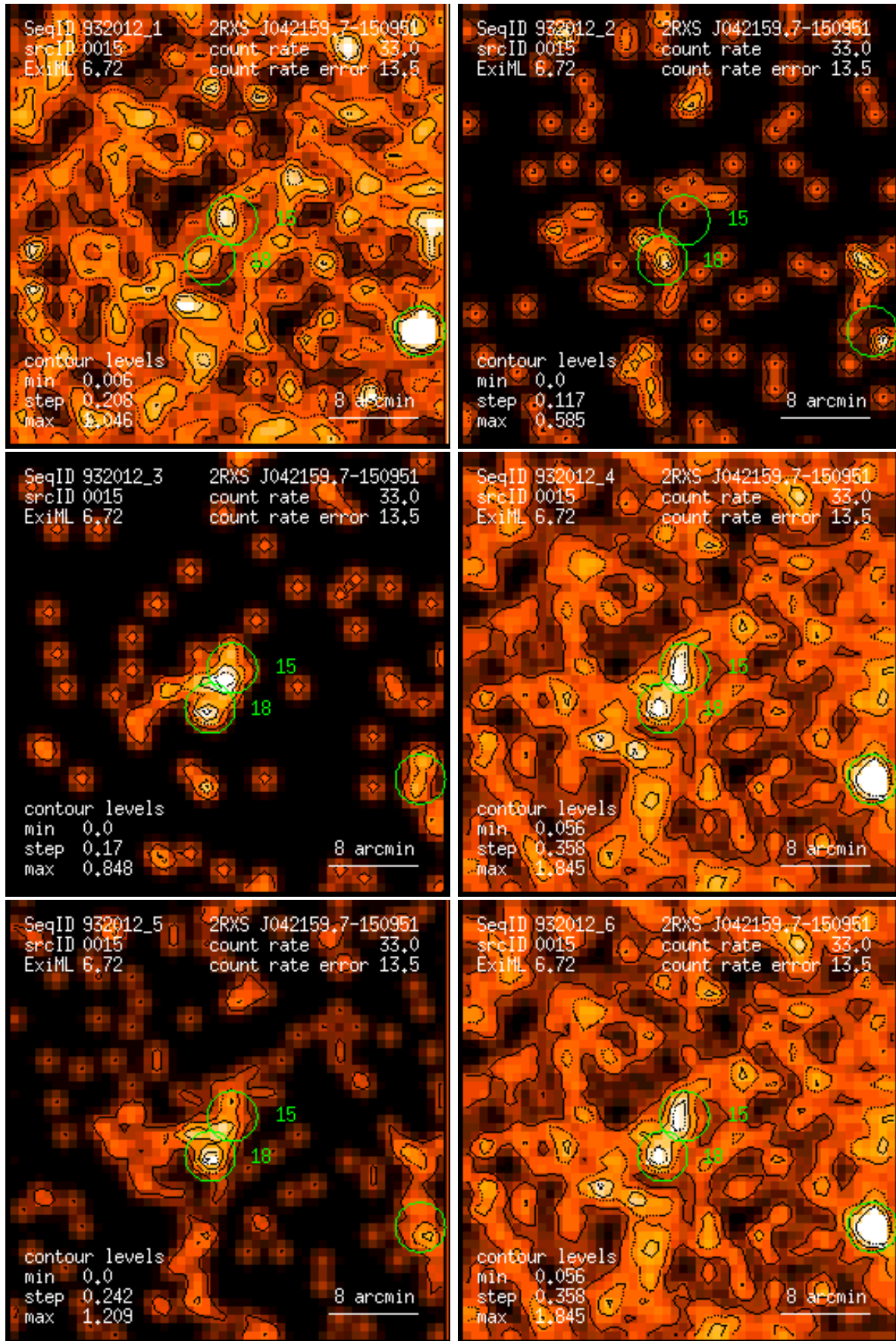
Figure 15: RASS 932012: detection 0015: band rate images, Gaussian filter: (1) PSPC channels 11 – 41, (2) 52 – 90, (3) 91 – 201, (4) 11 – 235, (5) 52 – 201, (6) 11 – 201. Broad band rates in counts/ks. Band rate contour levels in counts/ks/arcmin 2 .
