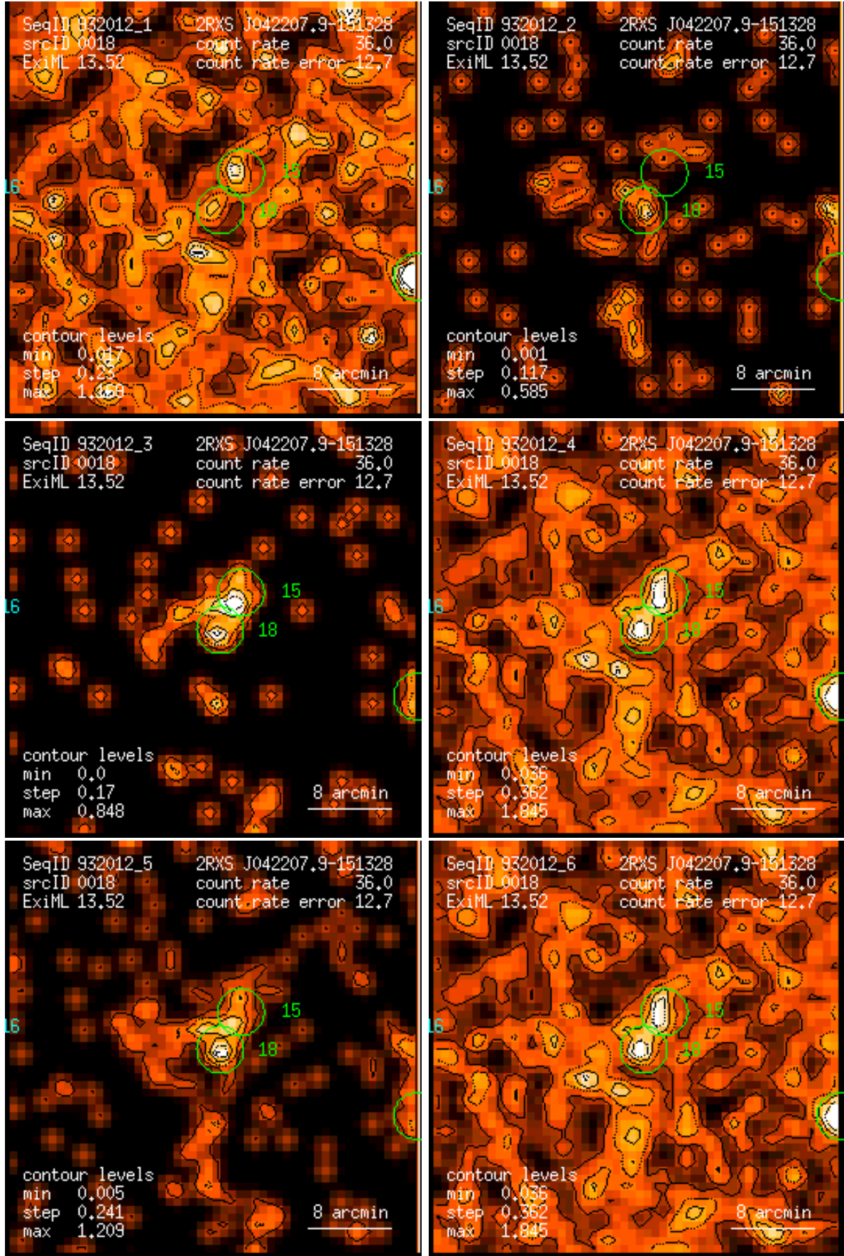
Figure 18: RASS 932012: detection 0018: band rate images, Gaussian filter: (1) PSPC channels 11 – 41, (2) 52 – 90, (3) 91 – 201, (4) 11 – 235, (5) 52 – 201, (6) 11 – 201. Broad band rates in counts/ks. Band rate contour levels in counts/ks/arcmin 2 .
