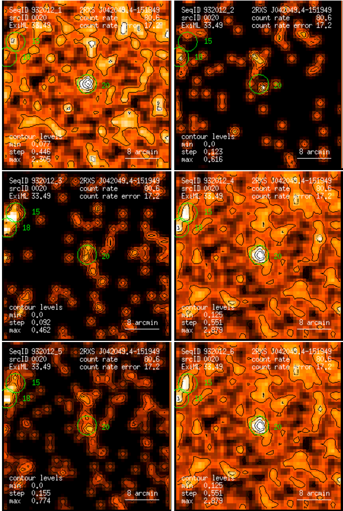
Figure 20: RASS 932012: detection 0020: band rate images, Gaussian filter: (1) PSPC channels 11 – 41, (2) 52 – 90, (3) 91 – 201, (4) 11 – 235, (5) 52 – 201, (6) 11 – 201. Broad band rates in counts/ks. Band rate contour levels in counts/ks/arcmin 2 .
